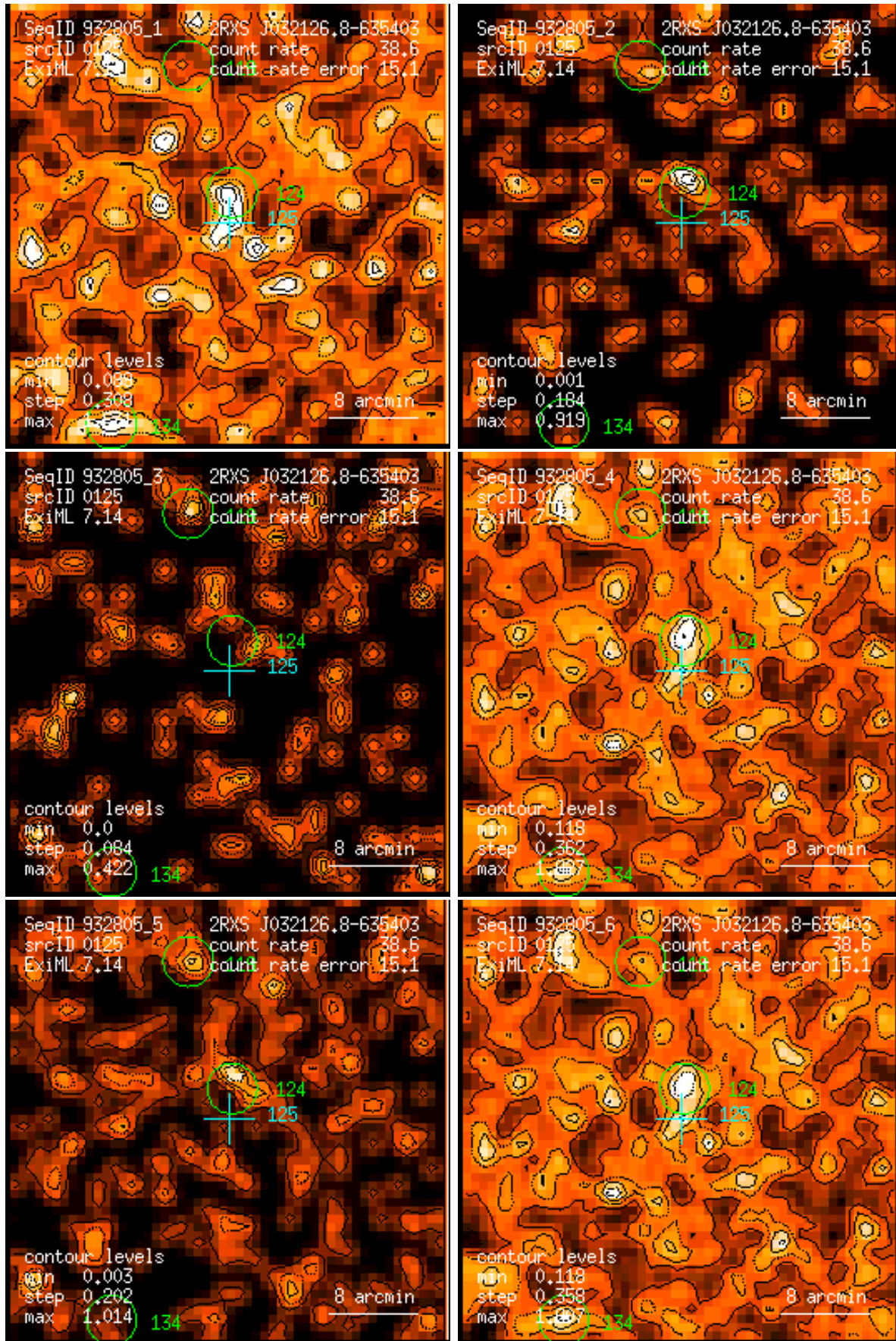
Figure 125: RASS 932805: detection 0125: band rate images, Gaussian filter: (1) PSPC channels 11 – 41, (2) 52 – 90, (3) 91 – 201, (4) 11 – 235, (5) 52 – 201, (6) 11 – 201. Broad band rates in counts/ks. Band rate contour levels in counts/ks/arcmin 2 .
