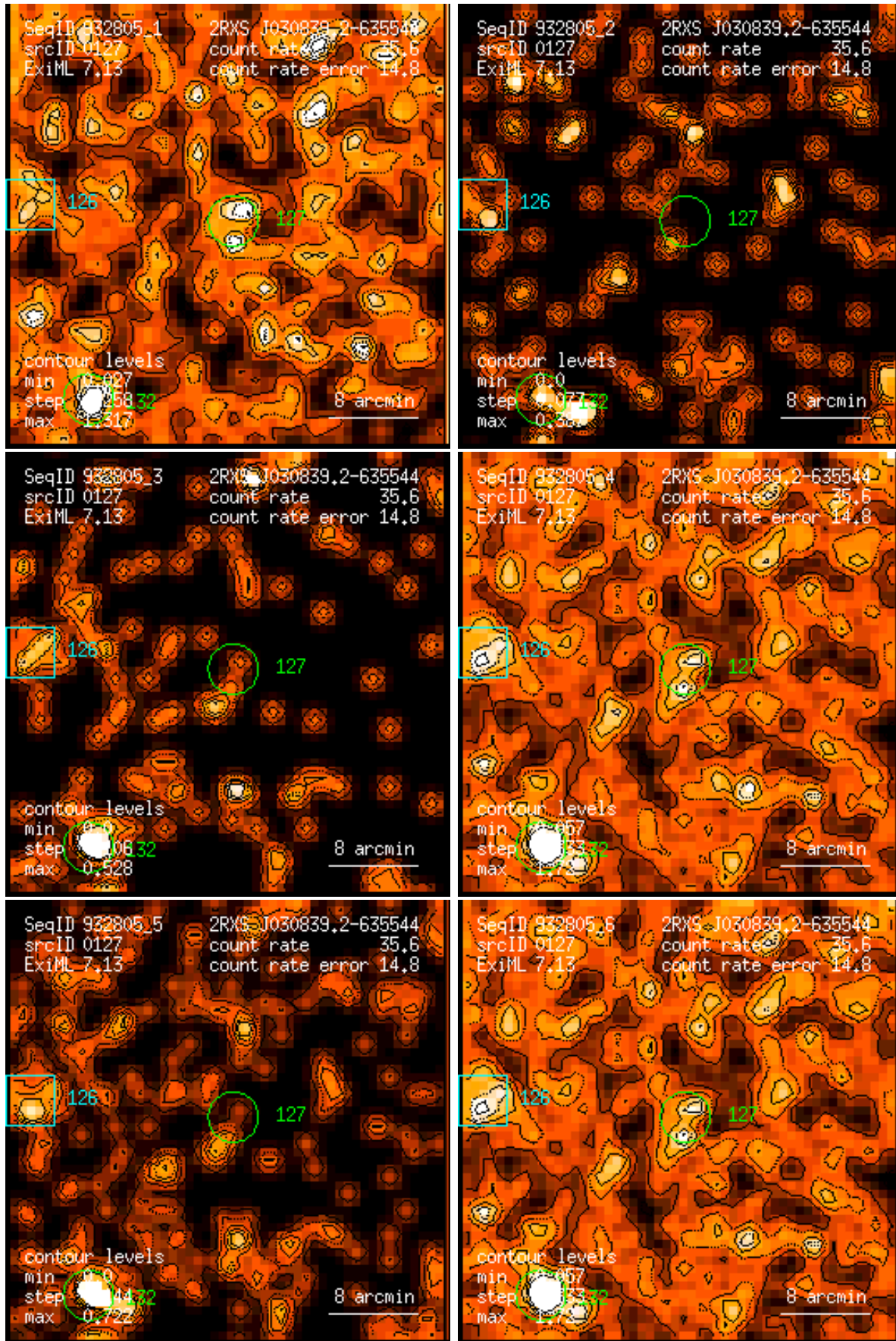
Figure 127: RASS 932805: detection 0127: band rate images, Gaussian filter: (1) PSPC channels 11 – 41, (2) 52 – 90, (3) 91 – 201, (4) 11 – 235, (5) 52 – 201, (6) 11 – 201. Broad band rates in counts/ks. Band rate contour levels in counts/ks/arcmin 2 .
