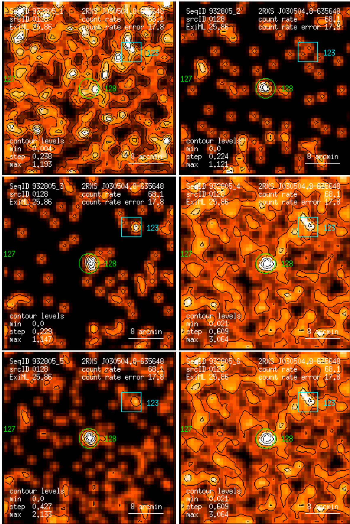
Figure 128: RASS 932805: detection 0128: band rate images, Gaussian filter: (1) PSPC channels 11 – 41, (2) 52 – 90, (3) 91 – 201, (4) 11 – 235, (5) 52 – 201, (6) 11 – 201. Broad band rates in counts/ks. Band rate contour levels in counts/ks/arcmin 2 .
