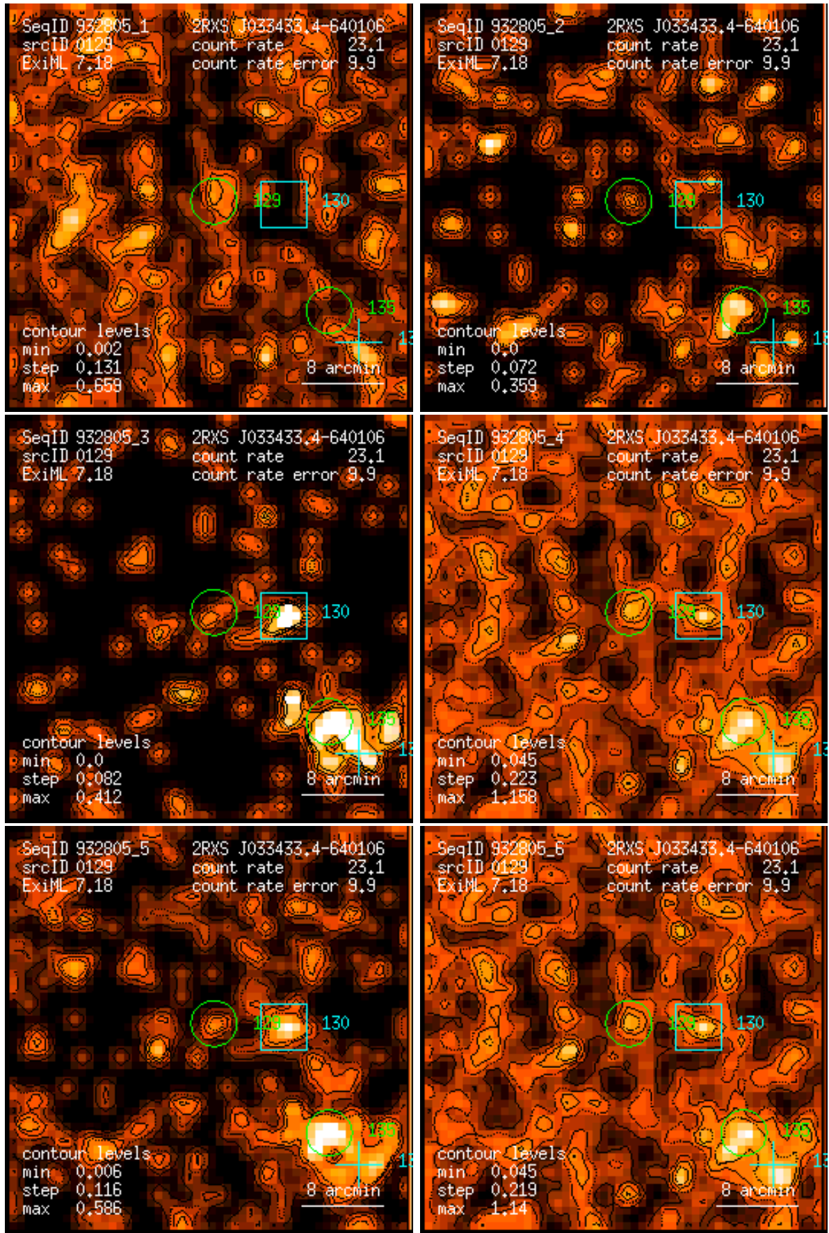
Figure 129: RASS 932805: detection 0129: band rate images, Gaussian filter: (1) PSPC channels 11 – 41, (2) 52 – 90, (3) 91 – 201, (4) 11 – 235, (5) 52 – 201, (6) 11 – 201. Broad band rates in counts/ks. Band rate contour levels in counts/ks/arcmin 2 .
