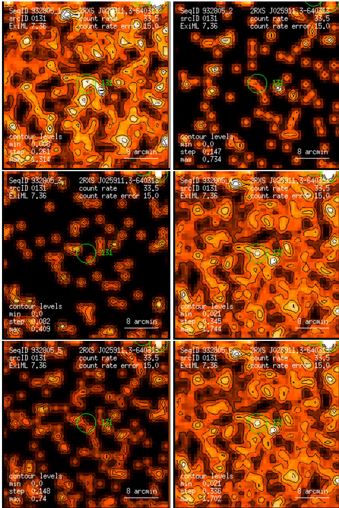
Figure 131: RASS 932805: detection 0131: band rate images, Gaussian filter: (1) PSPC channels 11 – 41, (2) 52 – 90, (3) 91 – 201, (4) 11 – 235, (5) 52 – 201, (6) 11 – 201. Broad band rates in counts/ks. Band rate contour levels in counts/ks/arcmin 2 .
