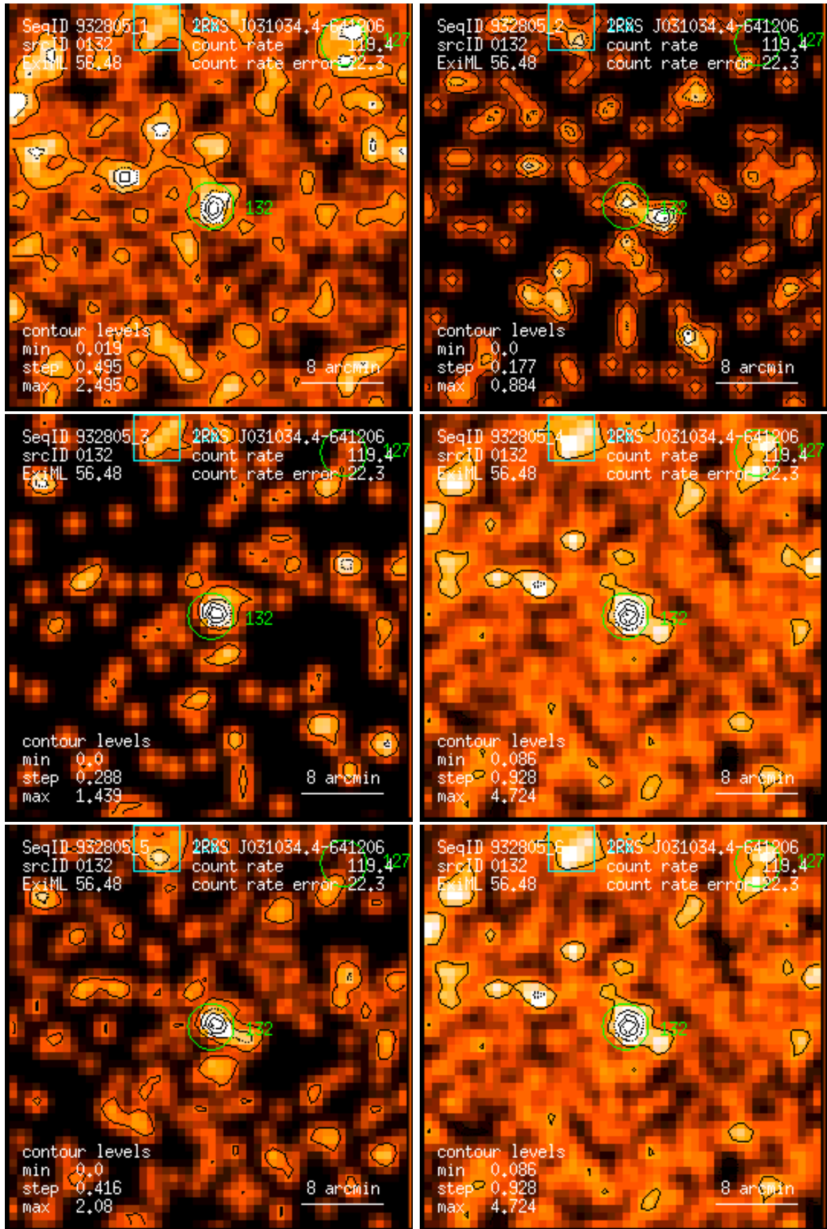
Figure 132: RASS 932805: detection 0132: band rate images, Gaussian filter: (1) PSPC channels 11 – 41, (2) 52 – 90, (3) 91 – 201, (4) 11 – 235, (5) 52 – 201, (6) 11 – 201. Broad band rates in counts/ks. Band rate contour levels in counts/ks/arcmin 2 .
