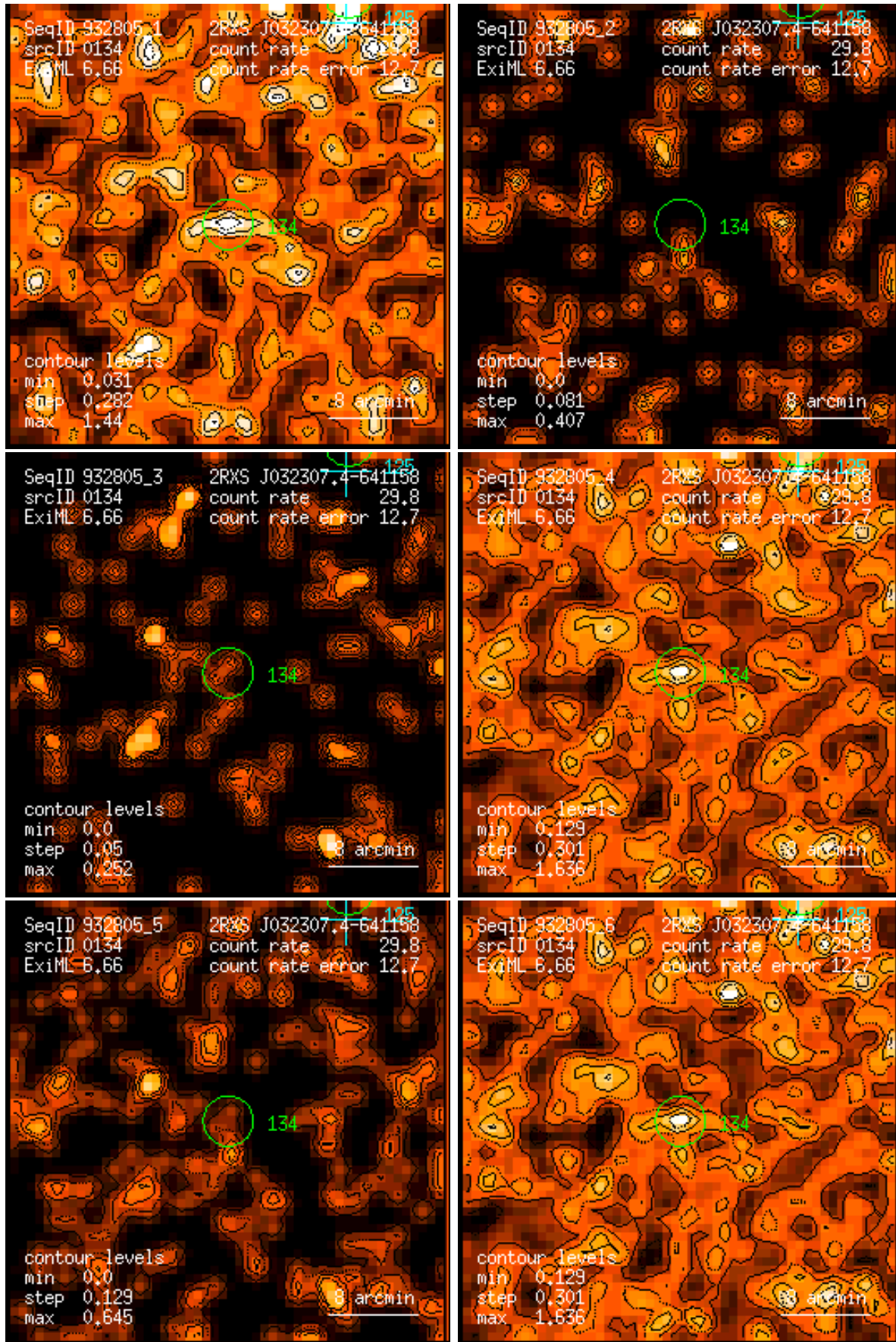
Figure 134: RASS 932805: detection 0134: band rate images, Gaussian filter: (1) PSPC channels 11 – 41, (2) 52 – 90, (3) 91 – 201, (4) 11 – 235, (5) 52 – 201, (6) 11 – 201. Broad band rates in counts/ks. Band rate contour levels in counts/ks/arcmin 2 .
