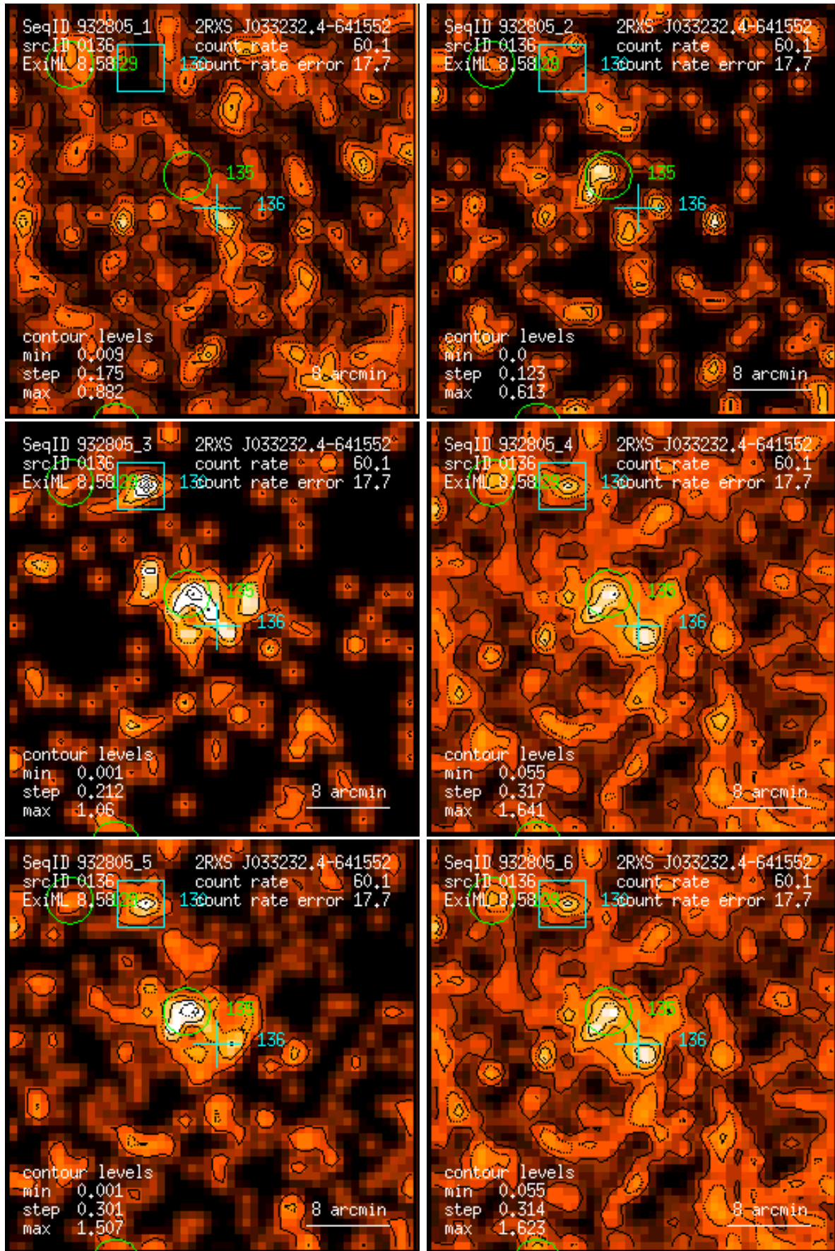
Figure 136: RASS 932805: detection 0136: band rate images, Gaussian filter: (1) PSPC channels 11 – 41, (2) 52 – 90, (3) 91 – 201, (4) 11 – 235, (5) 52 – 201, (6) 11 – 201. Broad band rates in counts/ks. Band rate contour levels in counts/ks/arcmin 2 .
