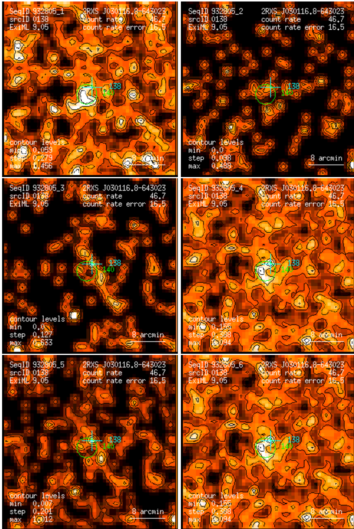
Figure 138: RASS 932805: detection 0138: band rate images, Gaussian filter: (1) PSPC channels 11 – 41, (2) 52 – 90, (3) 91 – 201, (4) 11 – 235, (5) 52 – 201, (6) 11 – 201. Broad band rates in counts/ks. Band rate contour levels in counts/ks/arcmin 2 .
