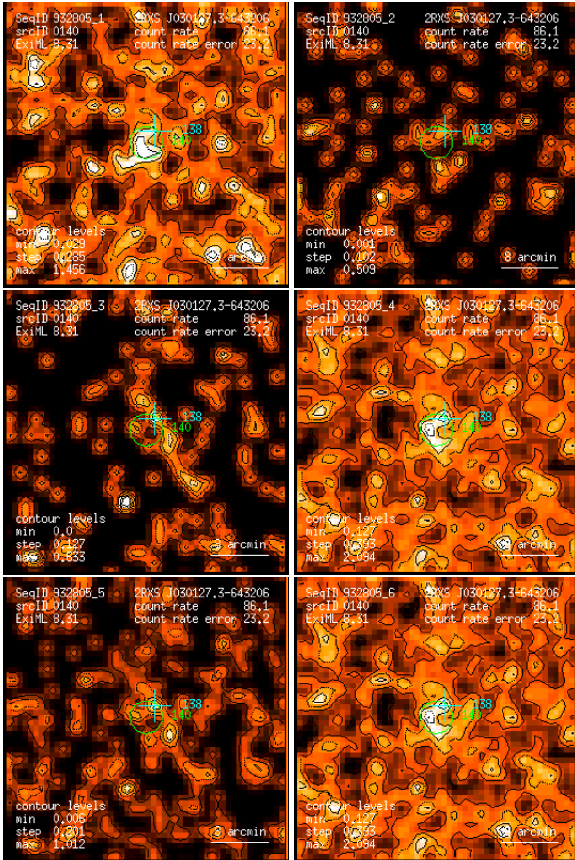
Figure 140: RASS 932805: detection 0140: band rate images, Gaussian filter: (1) PSPC channels 11 – 41, (2) 52 – 90, (3) 91 – 201, (4) 11 – 235, (5) 52 – 201, (6) 11 – 201. Broad band rates in counts/ks. Band rate contour levels in counts/ks/arcmin 2 .
