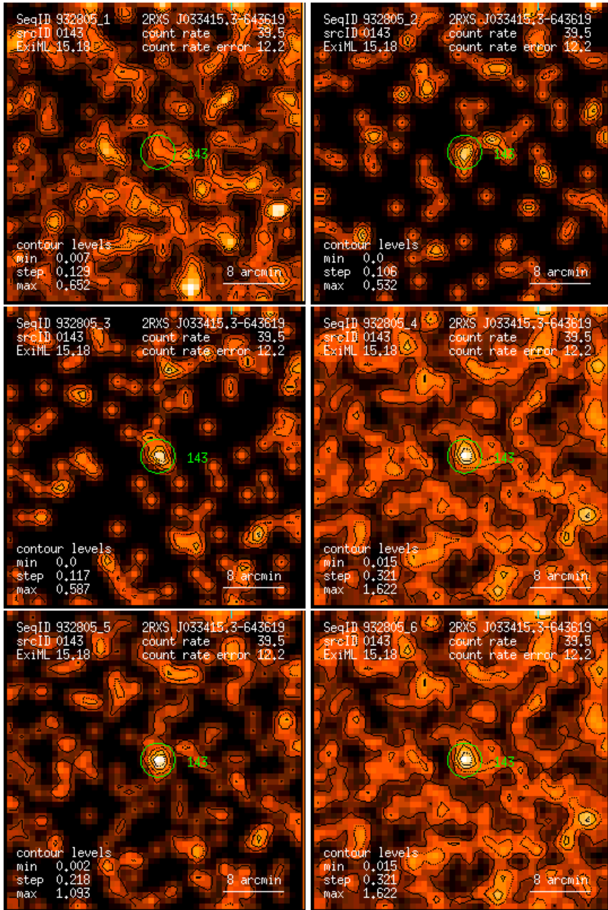
Figure 143: RASS 932805: detection 0143: band rate images, Gaussian filter: (1) PSPC channels 11 – 41, (2) 52 – 90, (3) 91 – 201, (4) 11 – 235, (5) 52 – 201, (6) 11 – 201. Broad band rates in counts/ks. Band rate contour levels in counts/ks/arcmin 2 .
