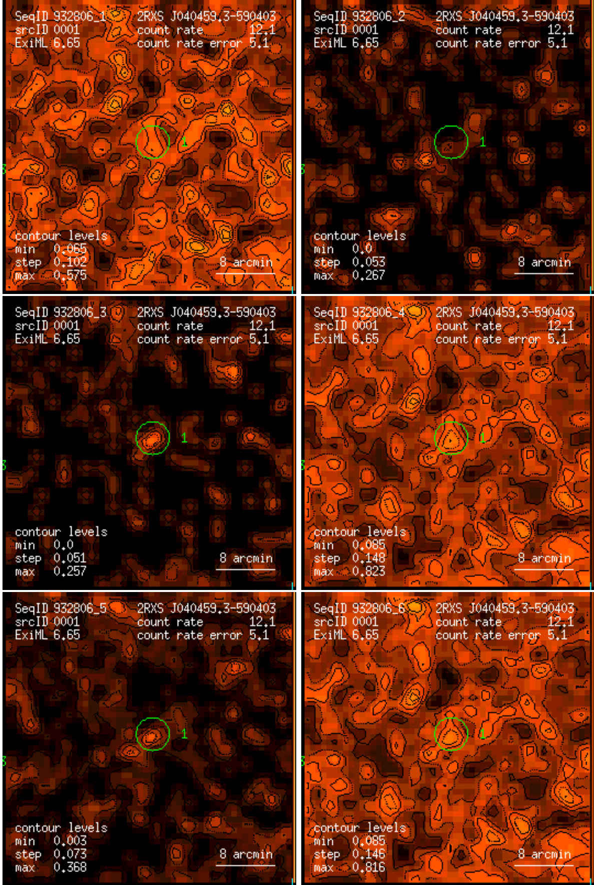
Figure 1: RASS 932806: detection 0001: band rate images, Gaussian filter: (1) PSPC channels 11 – 41, (2) 52 – 90, (3) 91 – 201, (4) 11 – 235, (5) 52 – 201, (6) 11 – 201. Broad band rates in counts/ks. Band rate contour levels in counts/ks/arcmin 2 .
