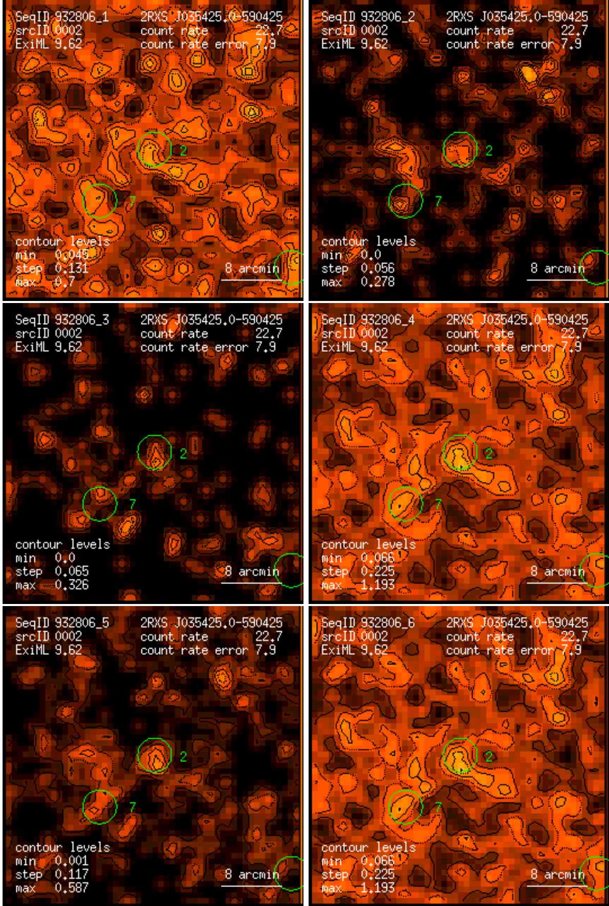
Figure 2: RASS 932806: detection 0002: band rate images, Gaussian filter: (1) PSPC channels 11 – 41, (2) 52 – 90, (3) 91 – 201, (4) 11 – 235, (5) 52 – 201, (6) 11 – 201. Broad band rates in counts/ks. Band rate contour levels in counts/ks/arcmin 2 .
