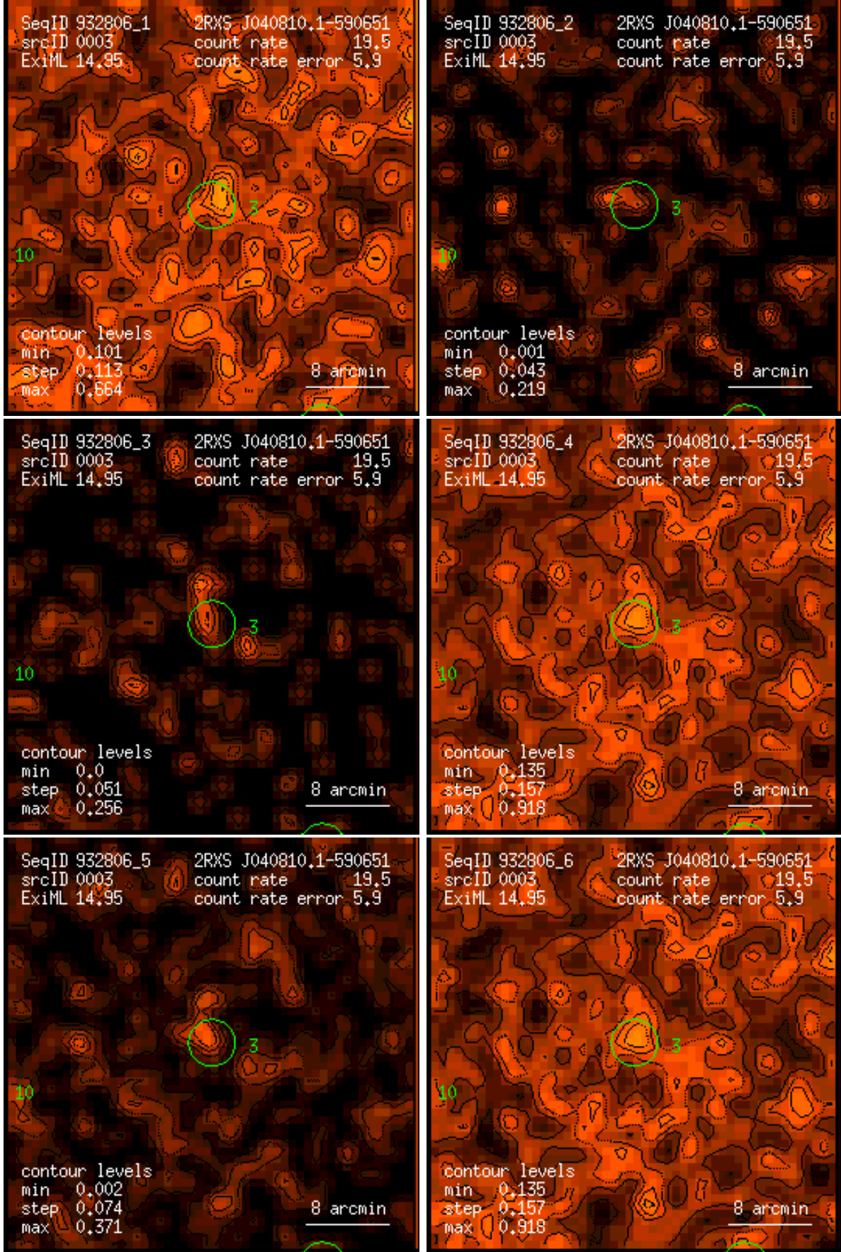
Figure 3: RASS 932806: detection 0003: band rate images, Gaussian filter: (1) PSPC channels 11 – 41, (2) 52 – 90, (3) 91 – 201, (4) 11 – 235, (5) 52 – 201, (6) 11 – 201. Broad band rates in counts/ks. Band rate contour levels in counts/ks/arcmin 2 .
