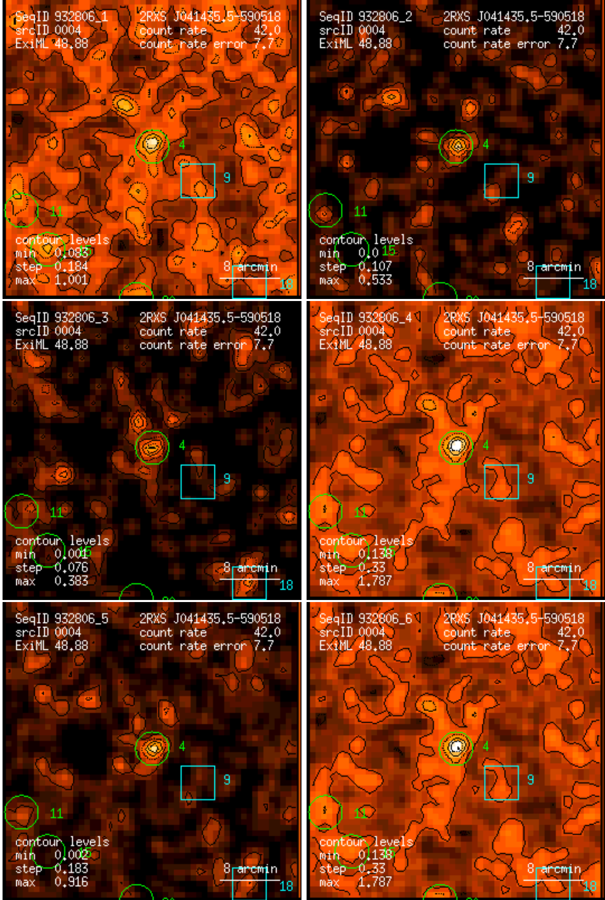
Figure 4: RASS 932806: detection 0004: band rate images, Gaussian filter: (1) PSPC channels 11 – 41, (2) 52 – 90, (3) 91 – 201, (4) 11 – 235, (5) 52 – 201, (6) 11 – 201. Broad band rates in counts/ks. Band rate contour levels in counts/ks/arcmin 2 .
