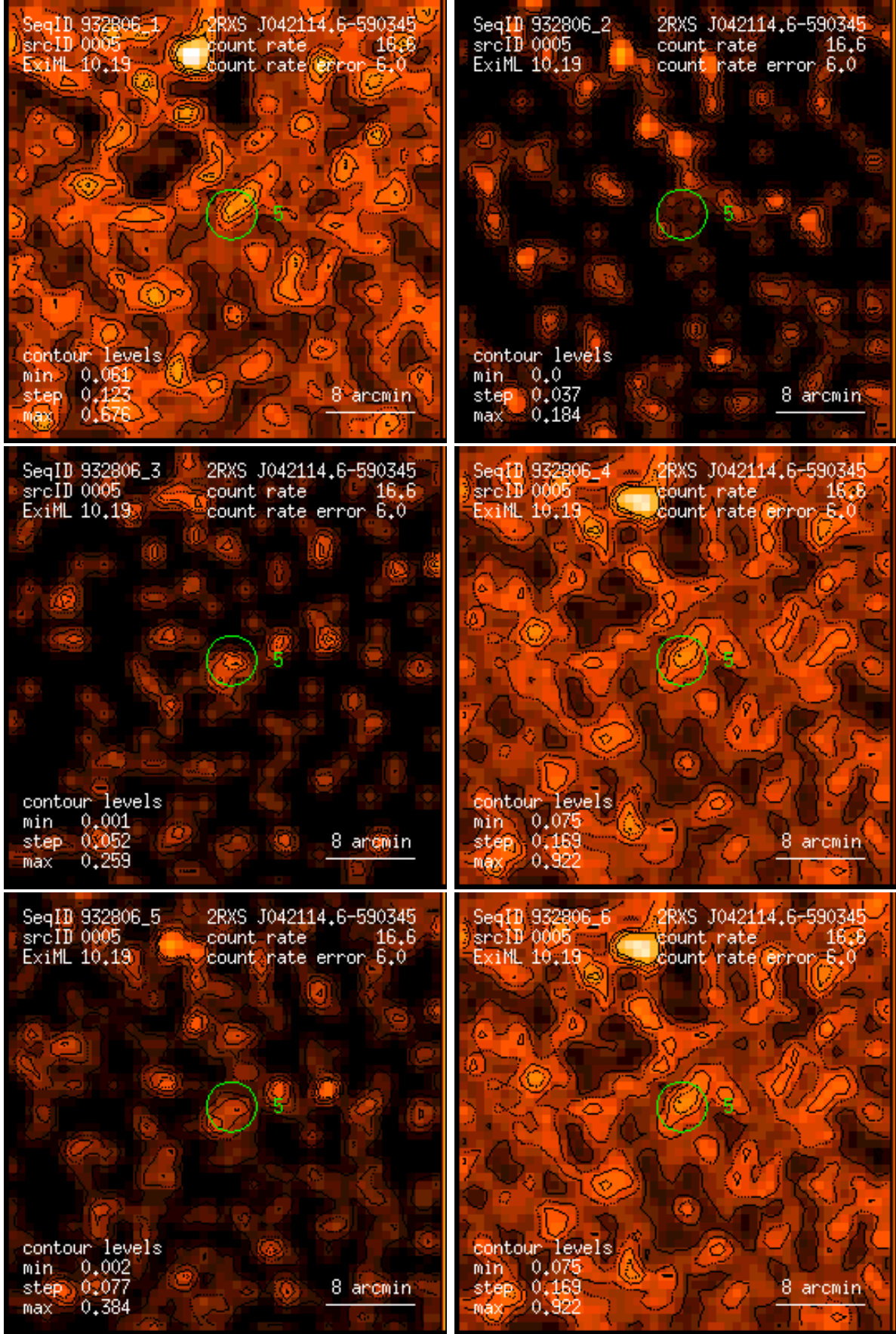
Figure 5: RASS 932806: detection 0005: band rate images, Gaussian filter: (1) PSPC channels 11 – 41, (2) 52 – 90, (3) 91 – 201, (4) 11 – 235, (5) 52 – 201, (6) 11 – 201. Broad band rates in counts/ks. Band rate contour levels in counts/ks/arcmin 2 .
