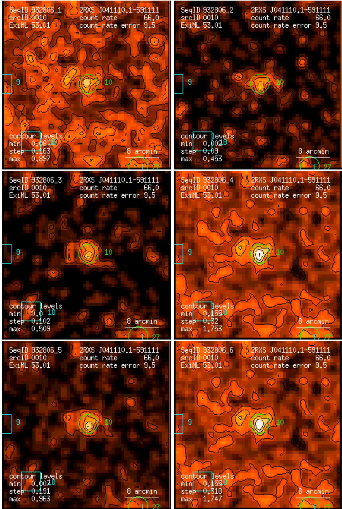
Figure 10: RASS 932806: detection 0010: band rate images, Gaussian filter: (1) PSPC channels 11 – 41, (2) 52 – 90, (3) 91 – 201, (4) 11 – 235, (5) 52 – 201, (6) 11 – 201. Broad band rates in counts/ks. Band rate contour levels in counts/ks/arcmin 2 .
