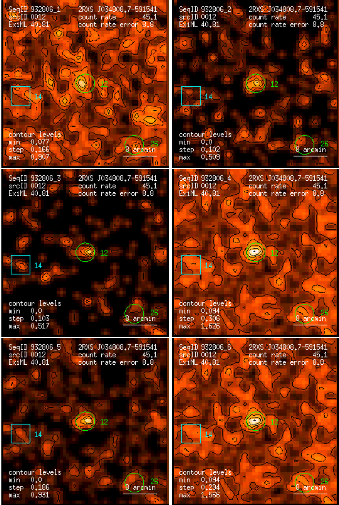
Figure 12: RASS 932806: detection 0012: band rate images, Gaussian filter: (1) PSPC channels 11 – 41, (2) 52 – 90, (3) 91 – 201, (4) 11 – 235, (5) 52 – 201, (6) 11 – 201. Broad band rates in counts/ks. Band rate contour levels in counts/ks/arcmin 2 .
