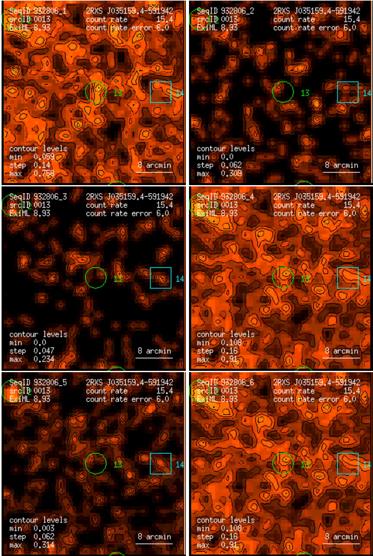
Figure 13: RASS 932806: detection 0013: band rate images, Gaussian filter: (1) PSPC channels 11 – 41, (2) 52 – 90, (3) 91 – 201, (4) 11 – 235, (5) 52 – 201, (6) 11 – 201. Broad band rates in counts/ks. Band rate contour levels in counts/ks/arcmin 2 .
