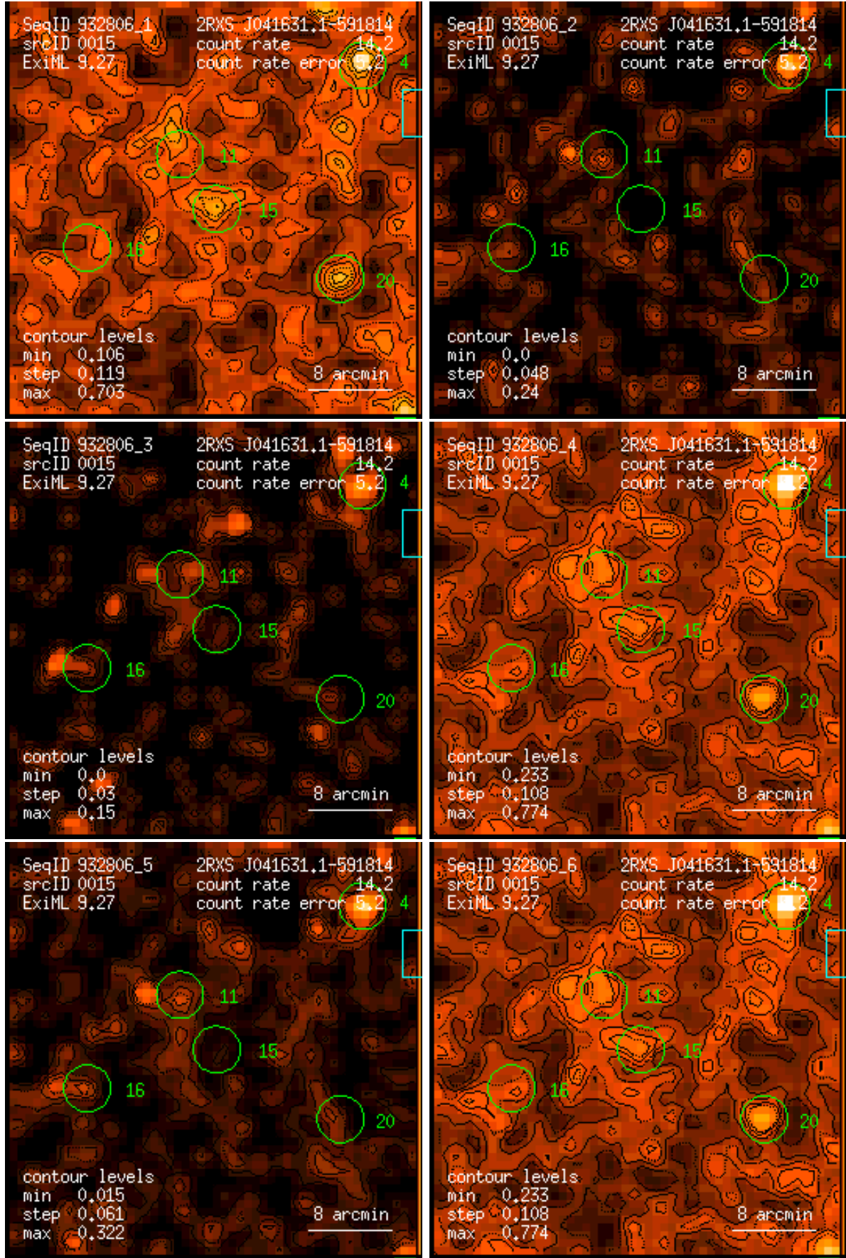
Figure 15: RASS 932806: detection 0015: band rate images, Gaussian filter: (1) PSPC channels 11 – 41, (2) 52 – 90, (3) 91 – 201, (4) 11 – 235, (5) 52 – 201, (6) 11 – 201. Broad band rates in counts/ks. Band rate contour levels in counts/ks/arcmin 2 .
