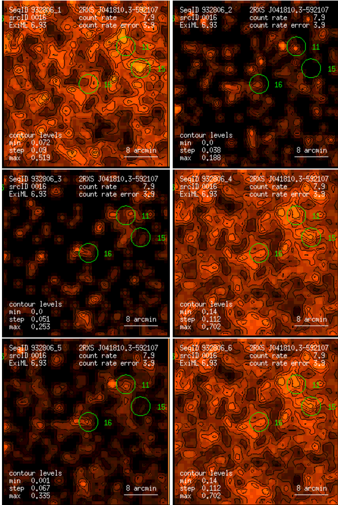
Figure 16: RASS 932806: detection 0016: band rate images, Gaussian filter: (1) PSPC channels 11 – 41, (2) 52 – 90, (3) 91 – 201, (4) 11 – 235, (5) 52 – 201, (6) 11 – 201. Broad band rates in counts/ks. Band rate contour levels in counts/ks/arcmin 2 .
