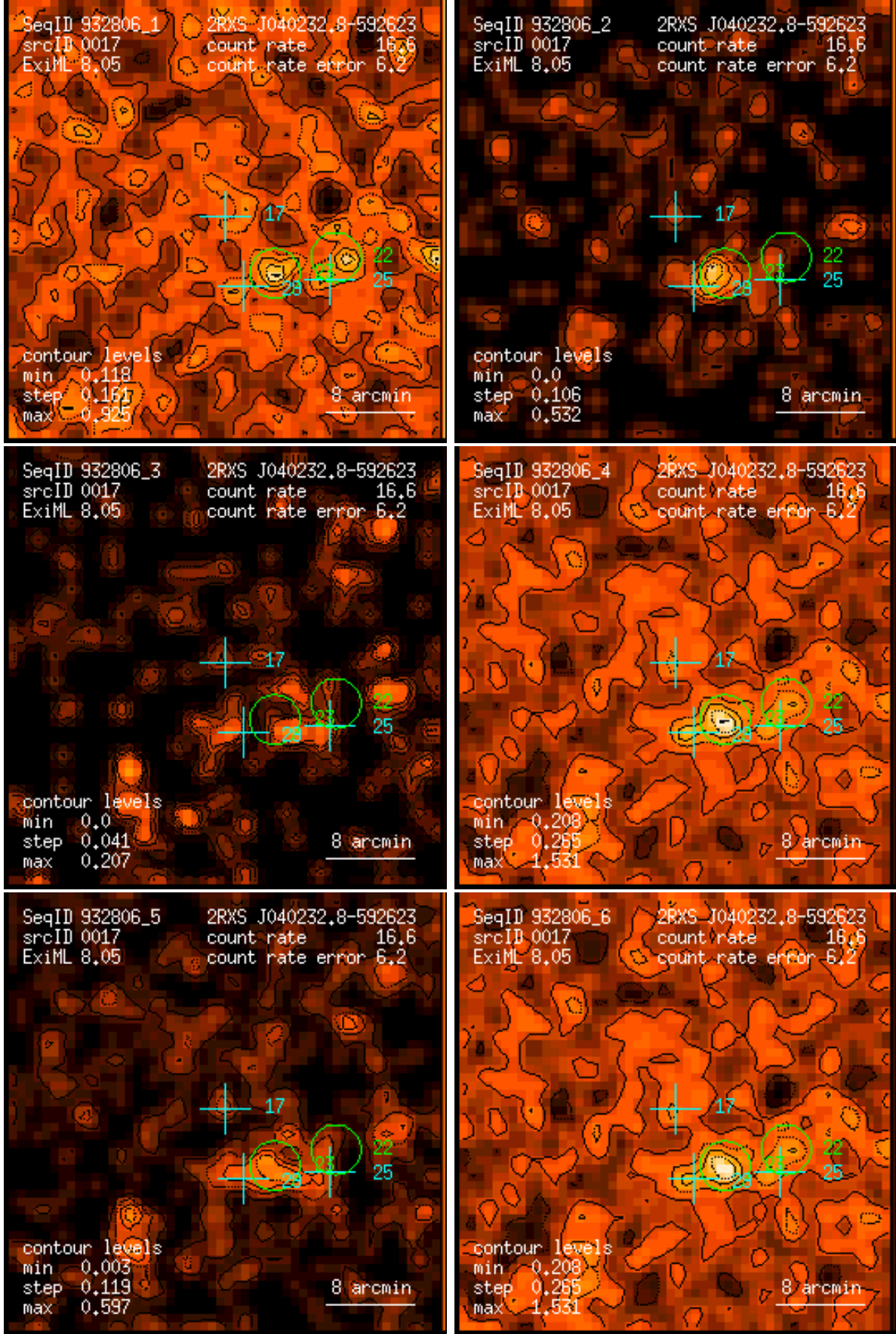
Figure 17: RASS 932806: detection 0017: band rate images, Gaussian filter: (1) PSPC channels 11 – 41, (2) 52 – 90, (3) 91 – 201, (4) 11 – 235, (5) 52 – 201, (6) 11 – 201. Broad band rates in counts/ks. Band rate contour levels in counts/ks/arcmin 2 .
