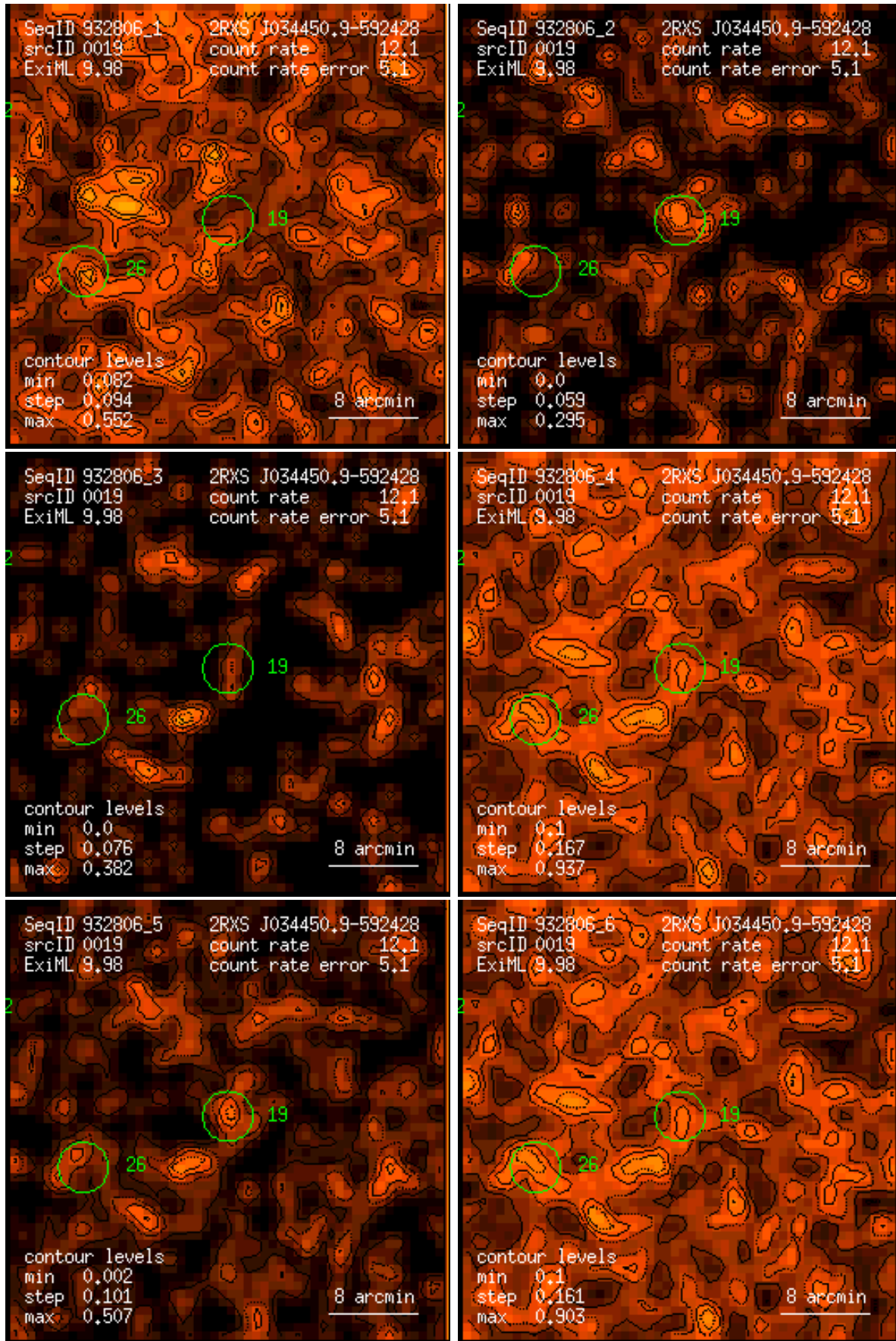
Figure 19: RASS 932806: detection 0019: band rate images, Gaussian filter: (1) PSPC channels 11 – 41, (2) 52 – 90, (3) 91 – 201, (4) 11 – 235, (5) 52 – 201, (6) 11 – 201. Broad band rates in counts/ks. Band rate contour levels in counts/ks/arcmin 2 .
