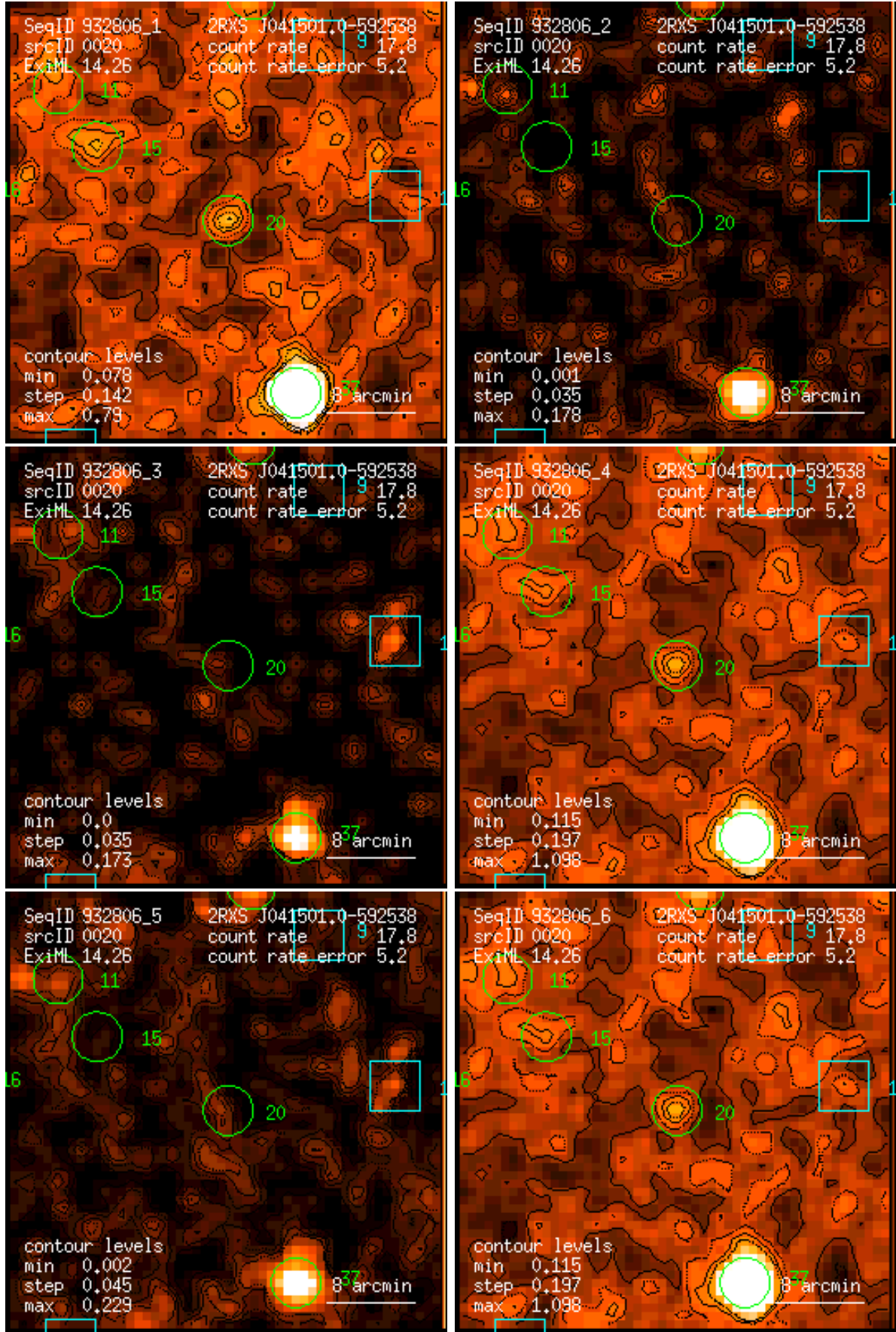
Figure 20: RASS 932806: detection 0020: band rate images, Gaussian filter: (1) PSPC channels 11 – 41, (2) 52 – 90, (3) 91 – 201, (4) 11 – 235, (5) 52 – 201, (6) 11 – 201. Broad band rates in counts/ks. Band rate contour levels in counts/ks/arcmin 2 .
