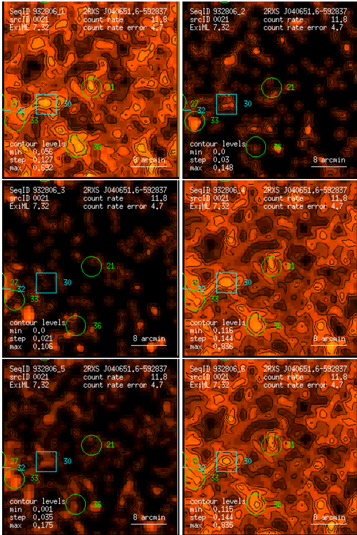
Figure 21: RASS 932806: detection 0021: band rate images, Gaussian filter: (1) PSPC channels 11 – 41, (2) 52 – 90, (3) 91 – 201, (4) 11 – 235, (5) 52 – 201, (6) 11 – 201. Broad band rates in counts/ks. Band rate contour levels in counts/ks/arcmin 2 .
