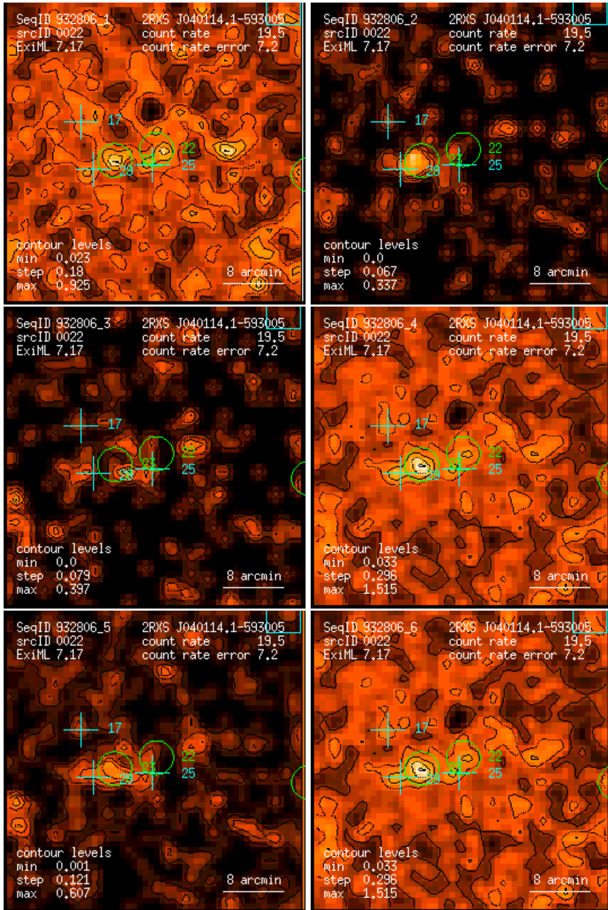
Figure 22: RASS 932806: detection 0022: band rate images, Gaussian filter: (1) PSPC channels 11 – 41, (2) 52 – 90, (3) 91 – 201, (4) 11 – 235, (5) 52 – 201, (6) 11 – 201. Broad band rates in counts/ks. Band rate contour levels in counts/ks/arcmin 2 .
