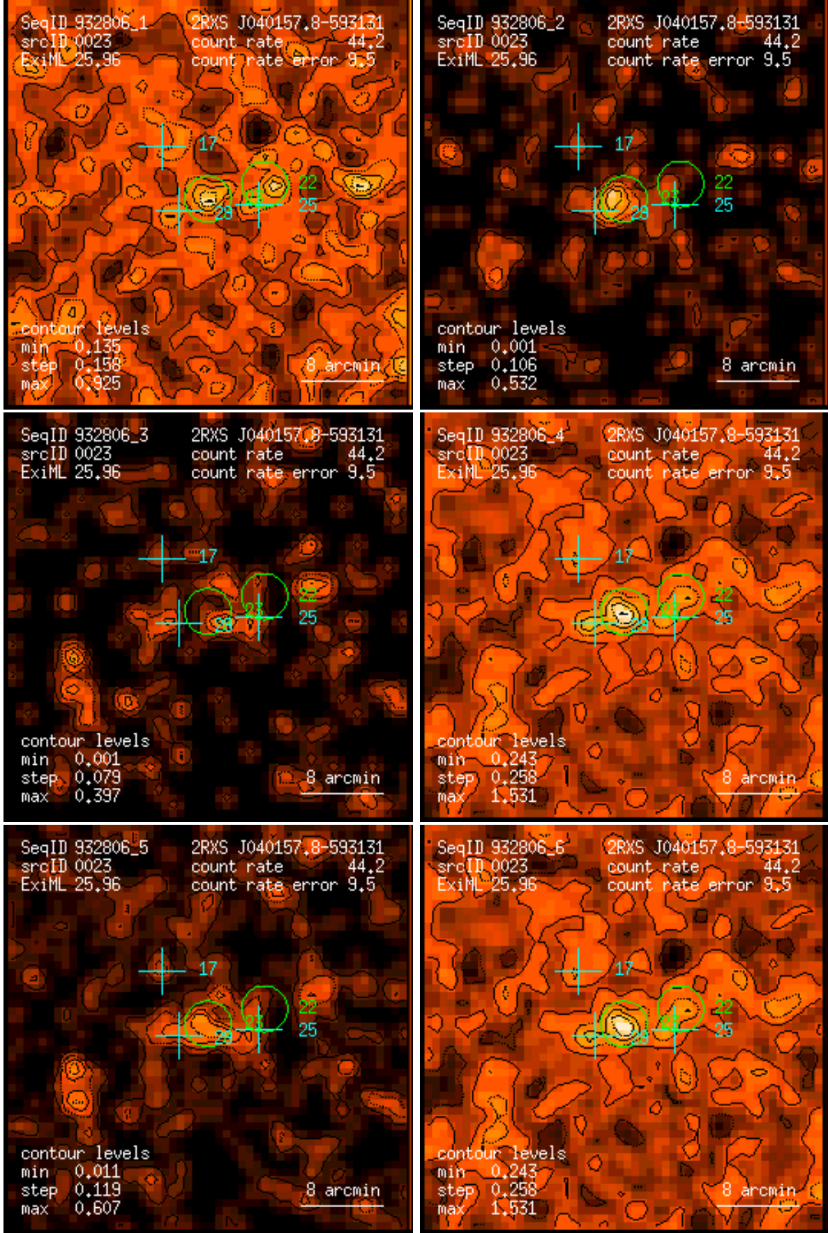
Figure 23: RASS 932806: detection 0023: band rate images, Gaussian filter: (1) PSPC channels 11 – 41, (2) 52 – 90, (3) 91 – 201, (4) 11 – 235, (5) 52 – 201, (6) 11 – 201. Broad band rates in counts/ks. Band rate contour levels in counts/ks/arcmin 2 .
