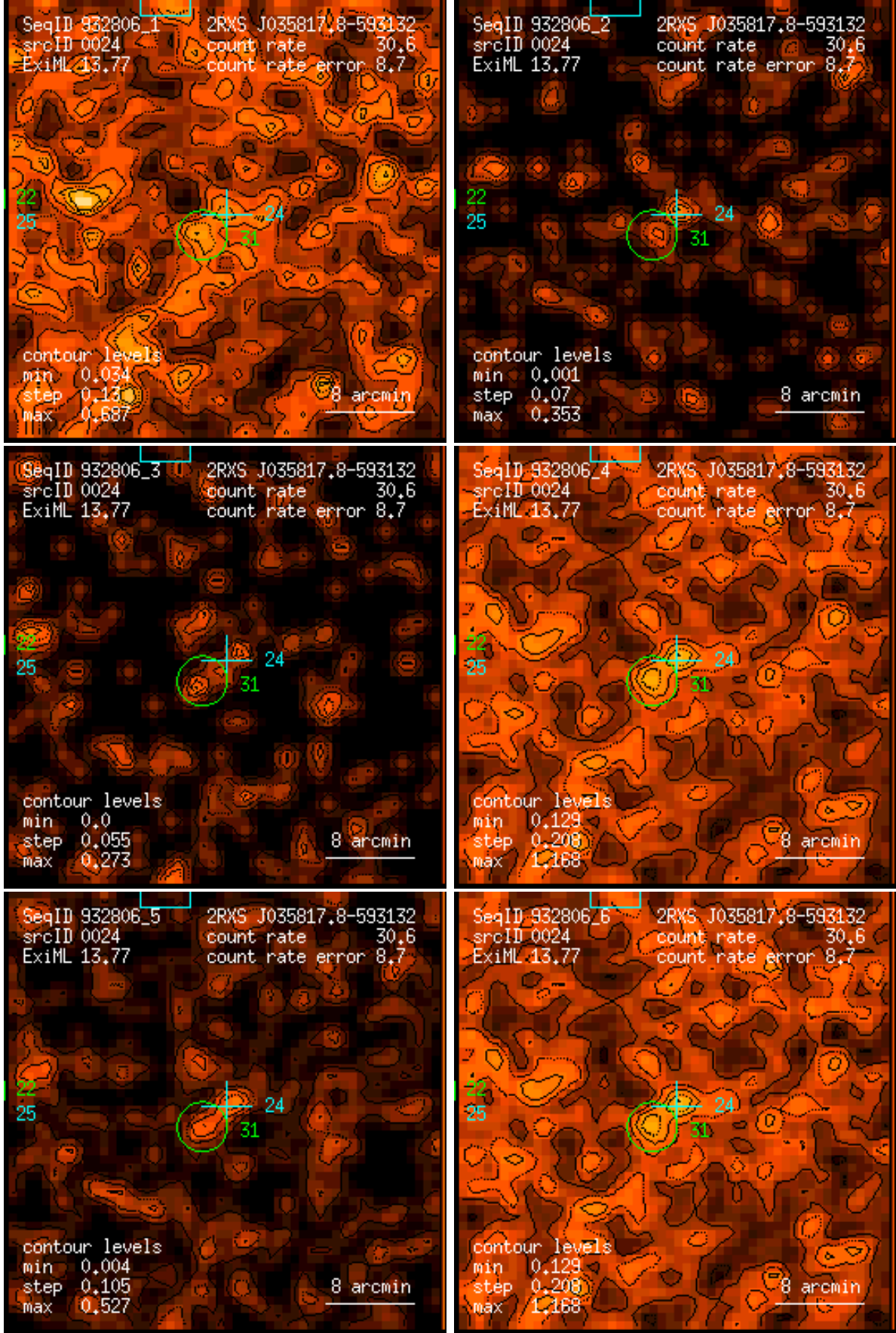
Figure 24: RASS 932806: detection 0024: band rate images, Gaussian filter: (1) PSPC channels 11 – 41, (2) 52 – 90, (3) 91 – 201, (4) 11 – 235, (5) 52 – 201, (6) 11 – 201. Broad band rates in counts/ks. Band rate contour levels in counts/ks/arcmin 2 .
