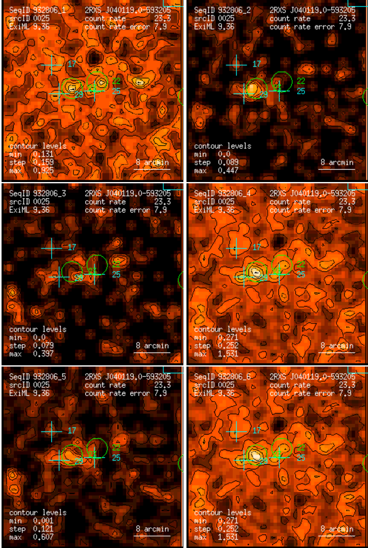
Figure 25: RASS 932806: detection 0025: band rate images, Gaussian filter: (1) PSPC channels 11 – 41, (2) 52 – 90, (3) 91 – 201, (4) 11 – 235, (5) 52 – 201, (6) 11 – 201. Broad band rates in counts/ks. Band rate contour levels in counts/ks/arcmin 2 .
