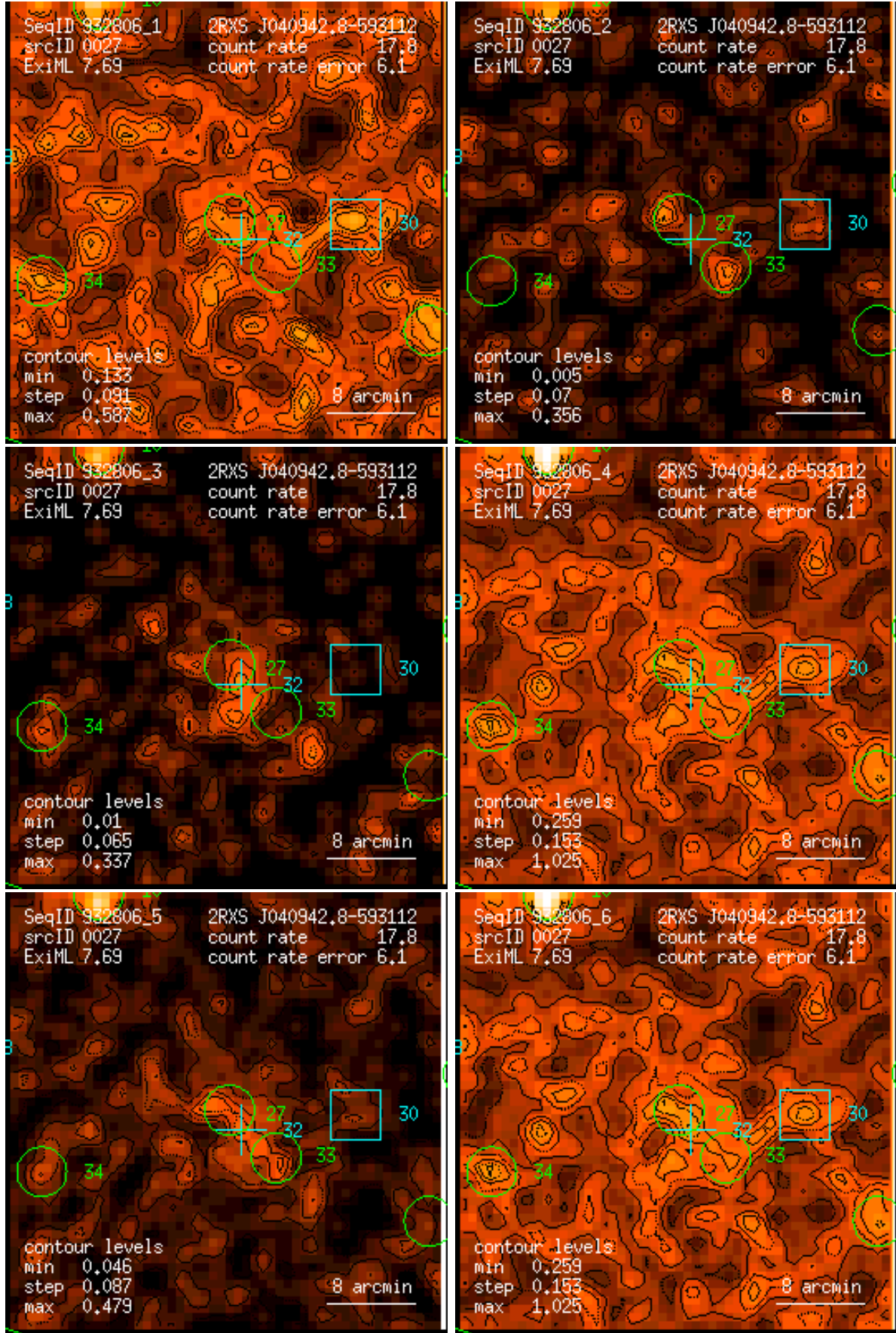
Figure 27: RASS 932806: detection 0027: band rate images, Gaussian filter: (1) PSPC channels 11 – 41, (2) 52 – 90, (3) 91 – 201, (4) 11 – 235, (5) 52 – 201, (6) 11 – 201. Broad band rates in counts/ks. Band rate contour levels in counts/ks/arcmin 2 .
