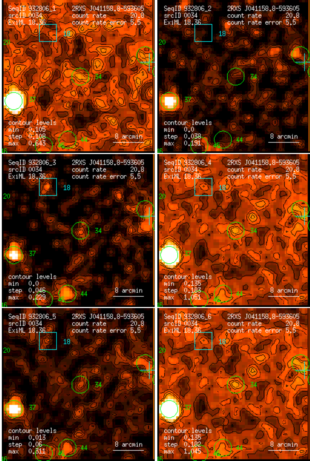
Figure 34: RASS 932806: detection 0034: band rate images, Gaussian filter: (1) PSPC channels 11 – 41, (2) 52 – 90, (3) 91 – 201, (4) 11 – 235, (5) 52 – 201, (6) 11 – 201. Broad band rates in counts/ks. Band rate contour levels in counts/ks/arcmin 2 .
