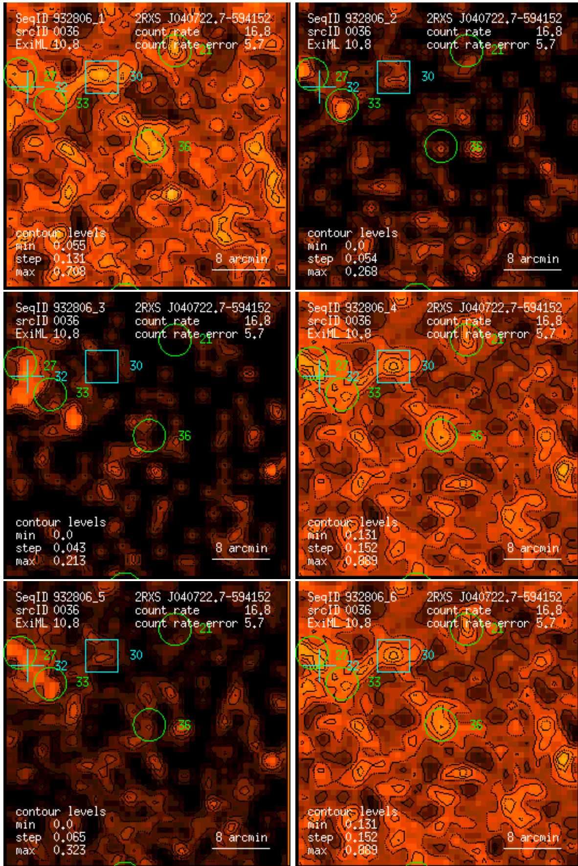
Figure 36: RASS 932806: detection 0036: band rate images, Gaussian filter: (1) PSPC channels 11 – 41, (2) 52 – 90, (3) 91 – 201, (4) 11 – 235, (5) 52 – 201, (6) 11 – 201. Broad band rates in counts/ks. Band rate contour levels in counts/ks/arcmin 2 .
