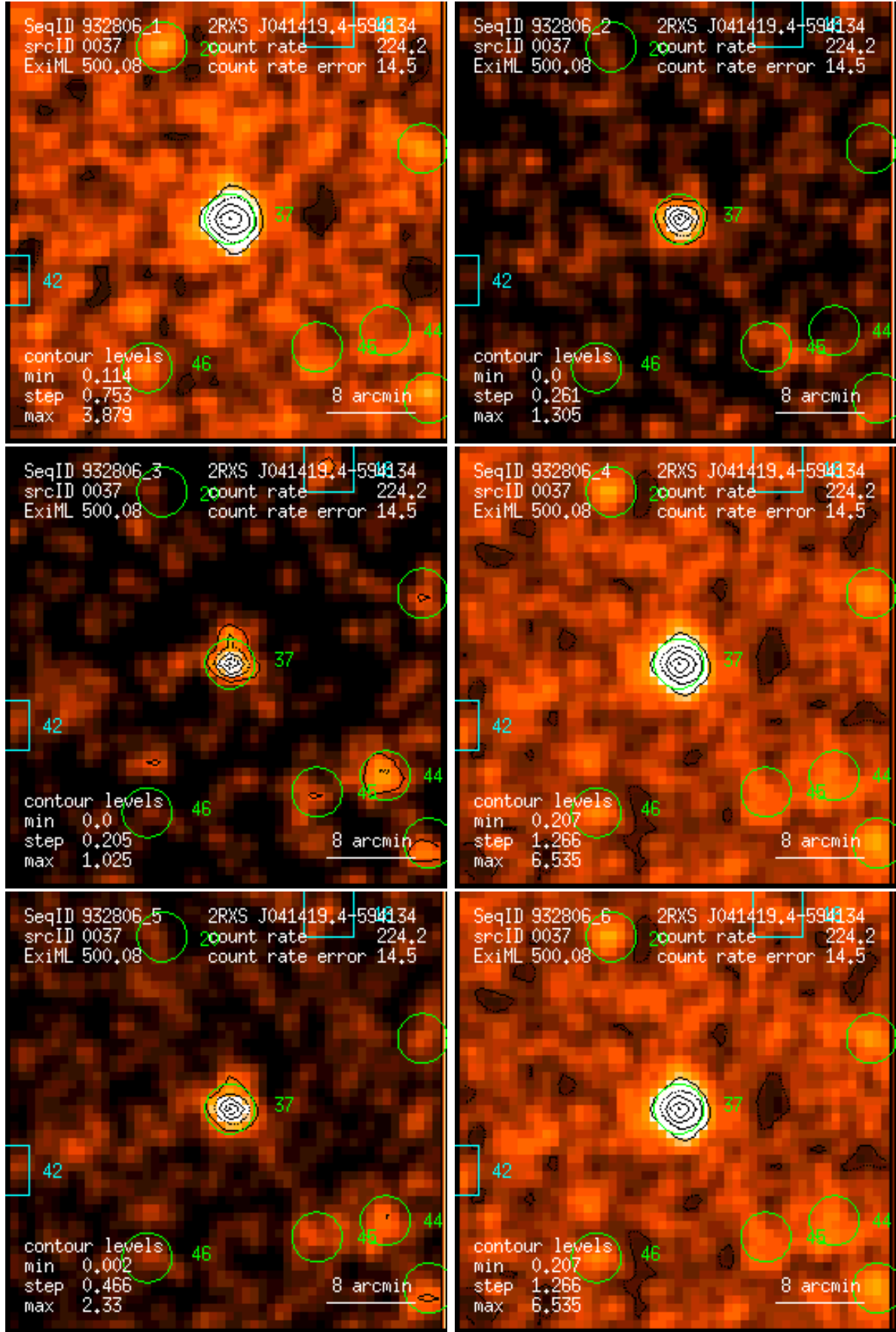
Figure 37: RASS 932806: detection 0037: band rate images, Gaussian filter: (1) PSPC channels 11 – 41, (2) 52 – 90, (3) 91 – 201, (4) 11 – 235, (5) 52 – 201, (6) 11 – 201. Broad band rates in counts/ks. Band rate contour levels in counts/ks/arcmin 2 .
