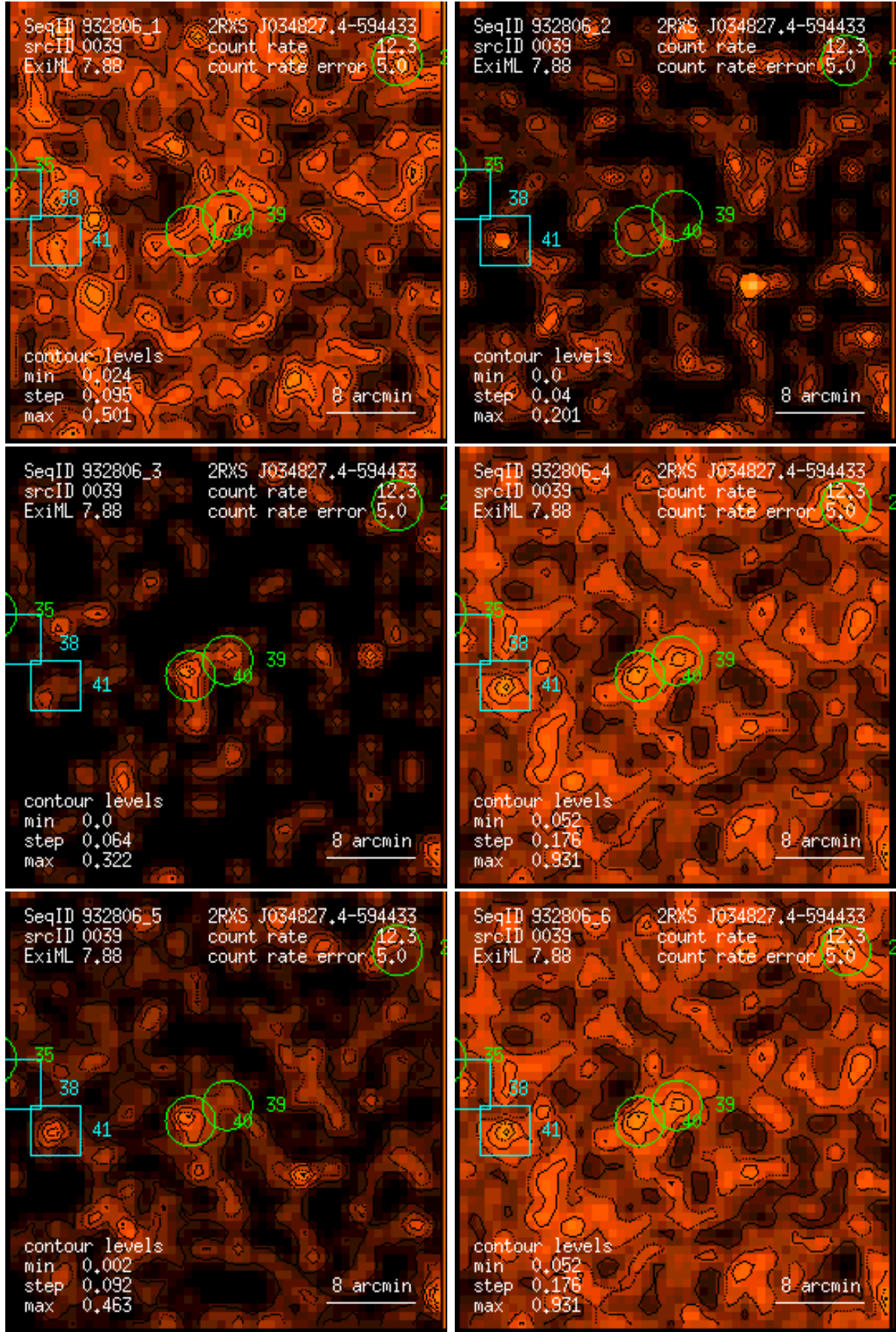
Figure 39: RASS 932806: detection 0039: band rate images, Gaussian filter: (1) PSPC channels 11 – 41, (2) 52 – 90, (3) 91 – 201, (4) 11 – 235, (5) 52 – 201, (6) 11 – 201. Broad band rates in counts/ks. Band rate contour levels in counts/ks/arcmin 2 .
