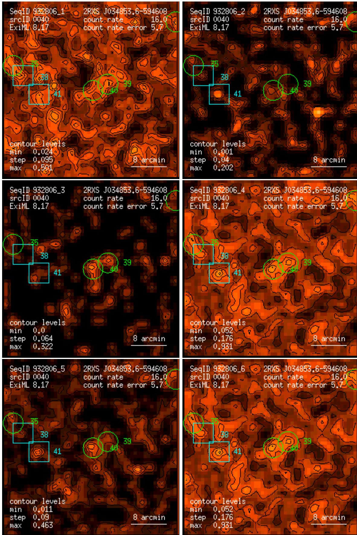
Figure 40: RASS 932806: detection 0040: band rate images, Gaussian filter: (1) PSPC channels 11 – 41, (2) 52 – 90, (3) 91 – 201, (4) 11 – 235, (5) 52 – 201, (6) 11 – 201. Broad band rates in counts/ks. Band rate contour levels in counts/ks/arcmin 2 .
