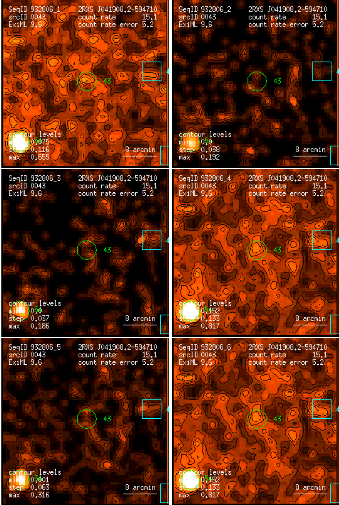
Figure 43: RASS 932806: detection 0043: band rate images, Gaussian filter: (1) PSPC channels 11 – 41, (2) 52 – 90, (3) 91 – 201, (4) 11 – 235, (5) 52 – 201, (6) 11 – 201. Broad band rates in counts/ks. Band rate contour levels in counts/ks/arcmin 2 .
