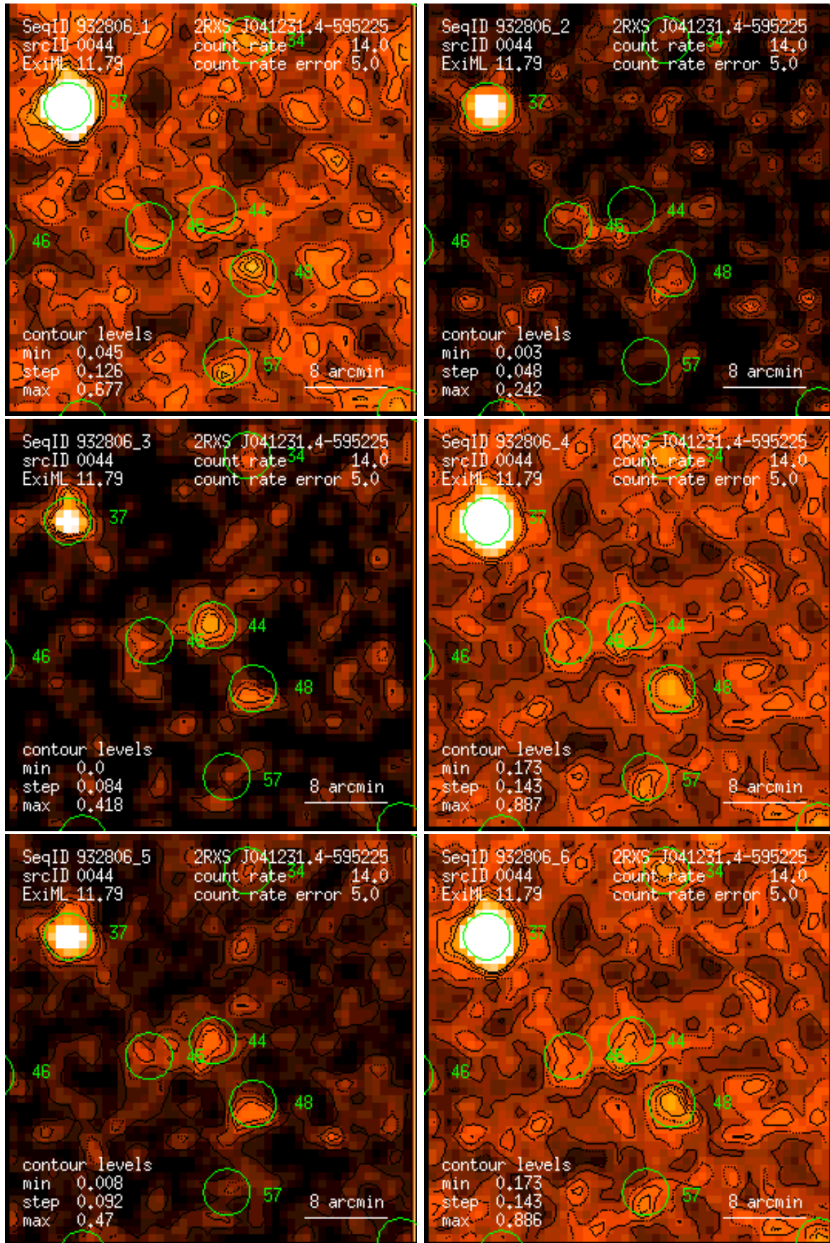
Figure 44: RASS 932806: detection 0044: band rate images, Gaussian filter: (1) PSPC channels 11 – 41, (2) 52 – 90, (3) 91 – 201, (4) 11 – 235, (5) 52 – 201, (6) 11 – 201. Broad band rates in counts/ks. Band rate contour levels in counts/ks/arcmin 2 .
