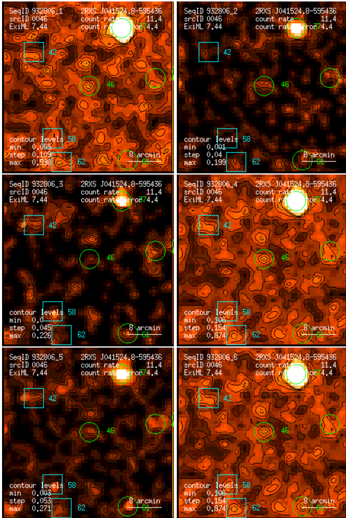
Figure 46: RASS 932806: detection 0046: band rate images, Gaussian filter: (1) PSPC channels 11 – 41, (2) 52 – 90, (3) 91 – 201, (4) 11 – 235, (5) 52 – 201, (6) 11 – 201. Broad band rates in counts/ks. Band rate contour levels in counts/ks/arcmin 2 .
