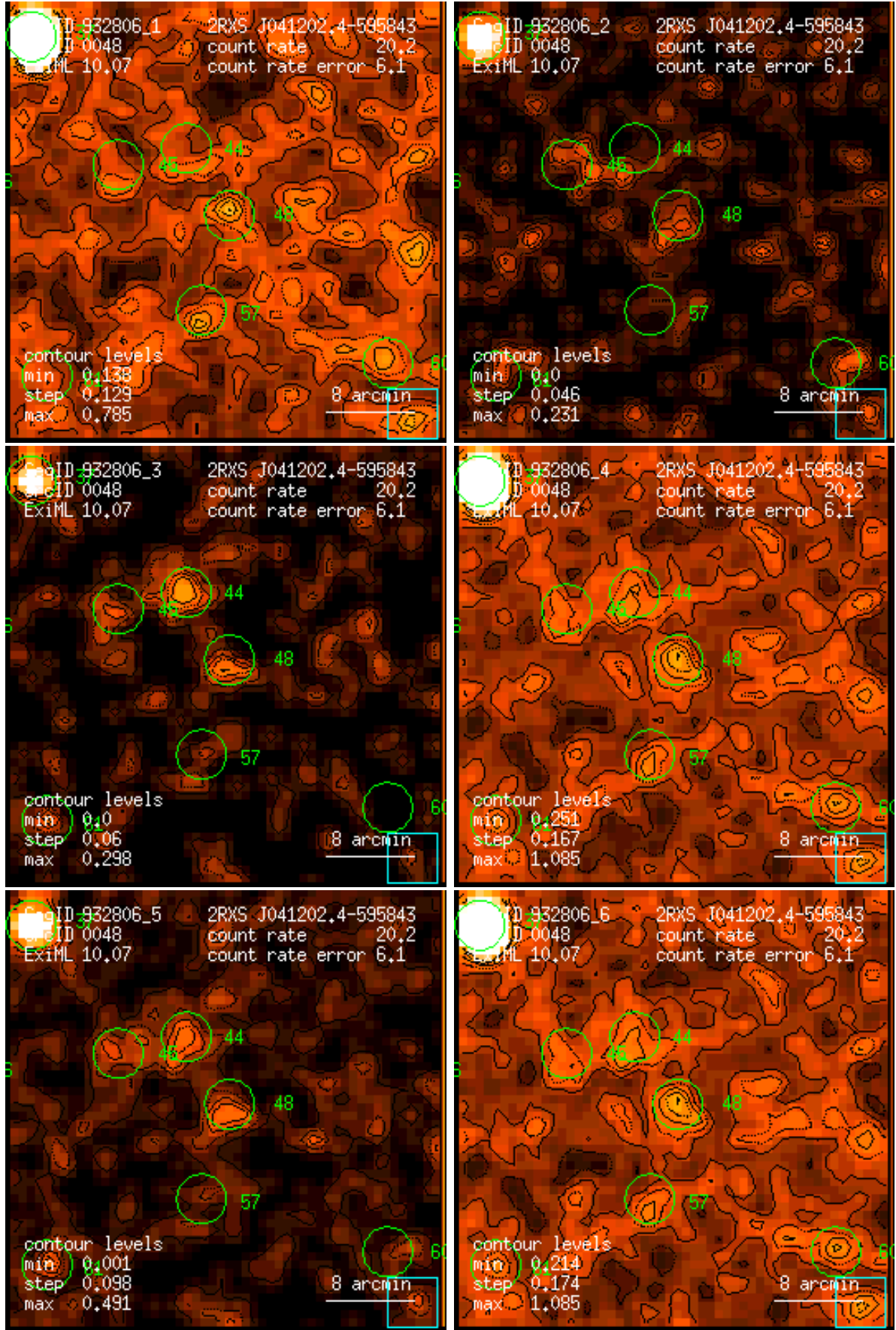
Figure 48: RASS 932806: detection 0048: band rate images, Gaussian filter: (1) PSPC channels 11 – 41, (2) 52 – 90, (3) 91 – 201, (4) 11 – 235, (5) 52 – 201, (6) 11 – 201. Broad band rates in counts/ks. Band rate contour levels in counts/ks/arcmin 2 .
