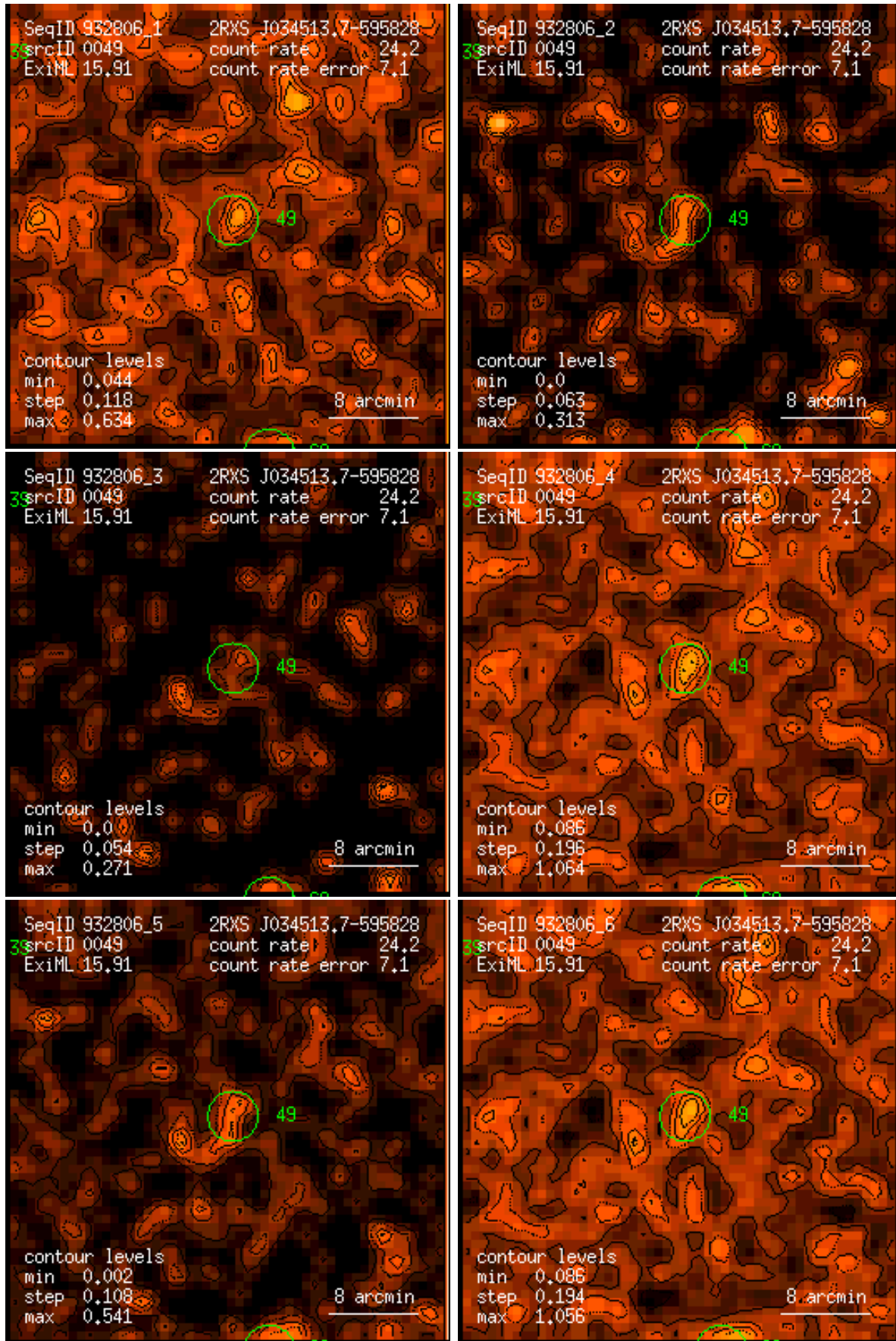
Figure 49: RASS 932806: detection 0049: band rate images, Gaussian filter: (1) PSPC channels 11 – 41, (2) 52 – 90, (3) 91 – 201, (4) 11 – 235, (5) 52 – 201, (6) 11 – 201. Broad band rates in counts/ks. Band rate contour levels in counts/ks/arcmin 2 .
