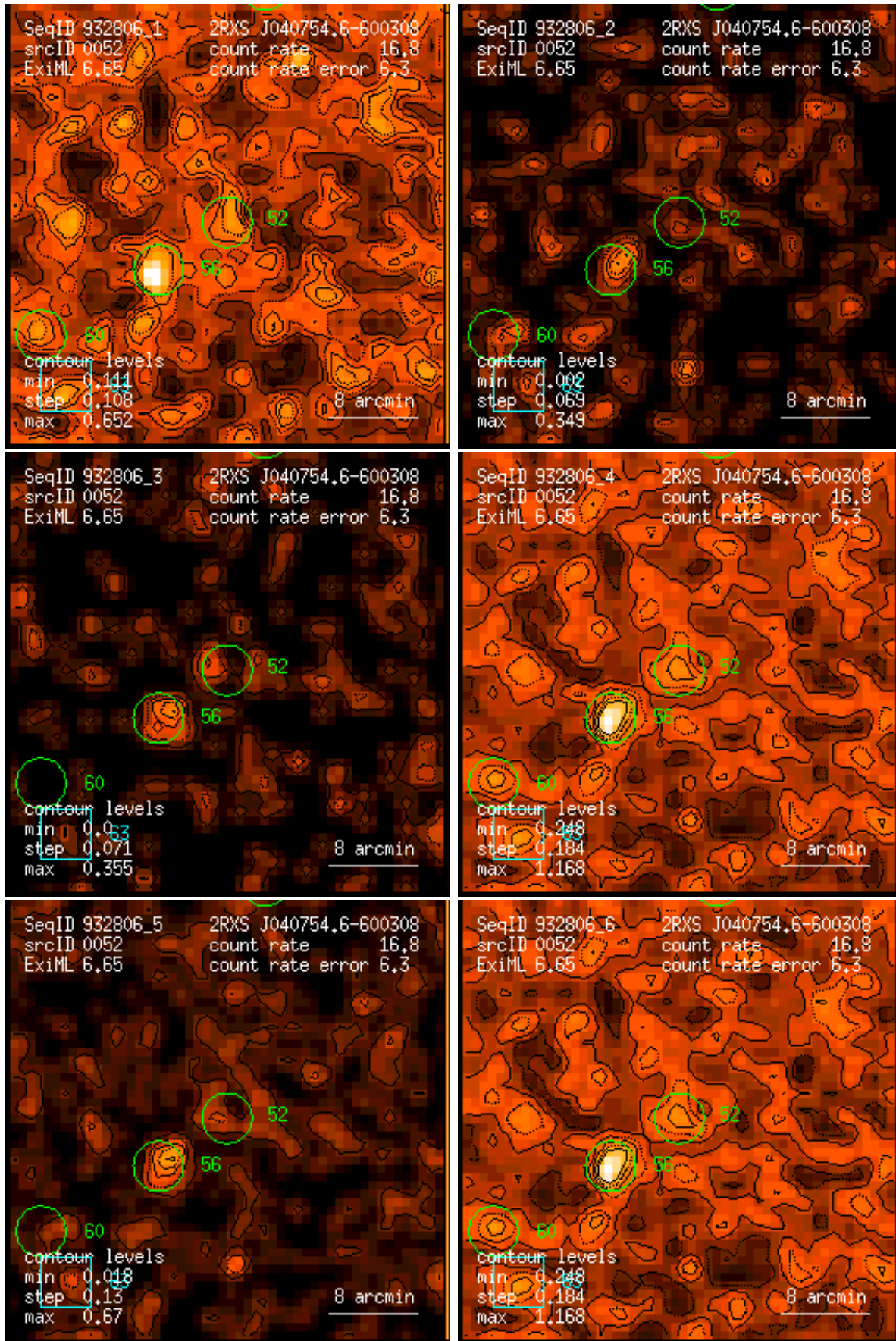
Figure 52: RASS 932806: detection 0052: band rate images, Gaussian filter: (1) PSPC channels 11 – 41, (2) 52 – 90, (3) 91 – 201, (4) 11 – 235, (5) 52 – 201, (6) 11 – 201. Broad band rates in counts/ks. Band rate contour levels in counts/ks/arcmin 2 .
