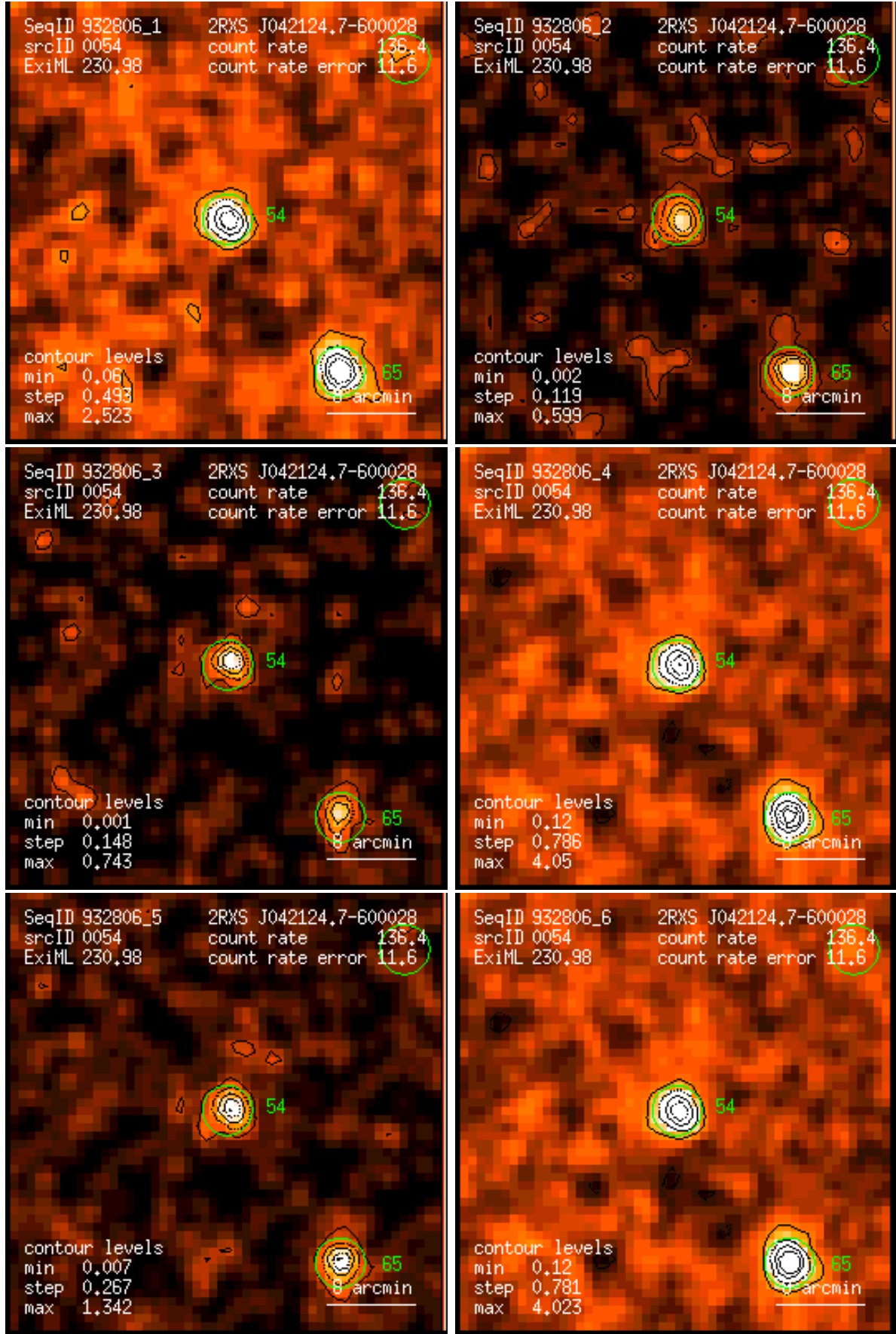
Figure 54: RASS 932806: detection 0054: band rate images, Gaussian filter: (1) PSPC channels 11 – 41, (2) 52 – 90, (3) 91 – 201, (4) 11 – 235, (5) 52 – 201, (6) 11 – 201. Broad band rates in counts/ks. Band rate contour levels in counts/ks/arcmin 2 .
