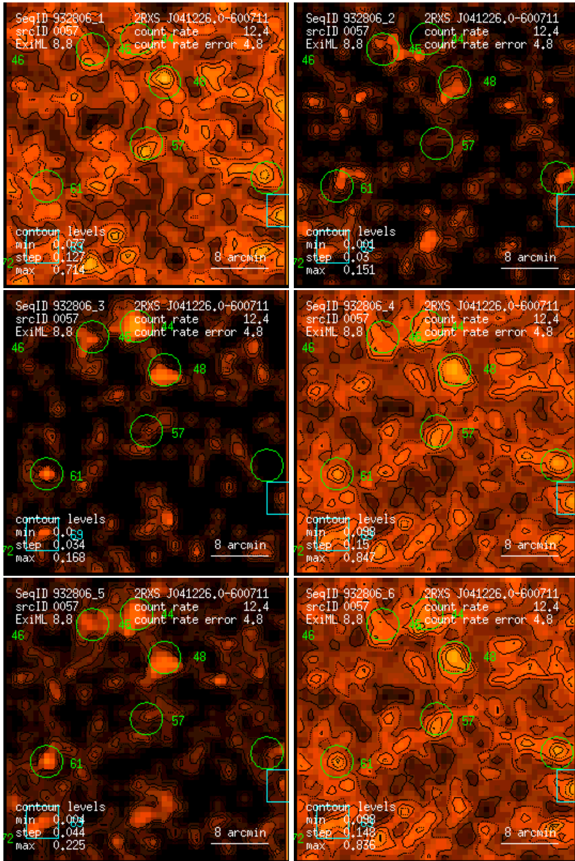
Figure 57: RASS 932806: detection 0057: band rate images, Gaussian filter: (1) PSPC channels 11 – 41, (2) 52 – 90, (3) 91 – 201, (4) 11 – 235, (5) 52 – 201, (6) 11 – 201. Broad band rates in counts/ks. Band rate contour levels in counts/ks/arcmin 2 .
