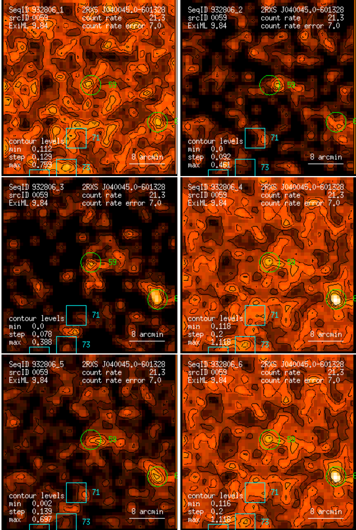
Figure 59: RASS 932806: detection 0059: band rate images, Gaussian filter: (1) PSPC channels 11 – 41, (2) 52 – 90, (3) 91 – 201, (4) 11 – 235, (5) 52 – 201, (6) 11 – 201. Broad band rates in counts/ks. Band rate contour levels in counts/ks/arcmin 2 .
