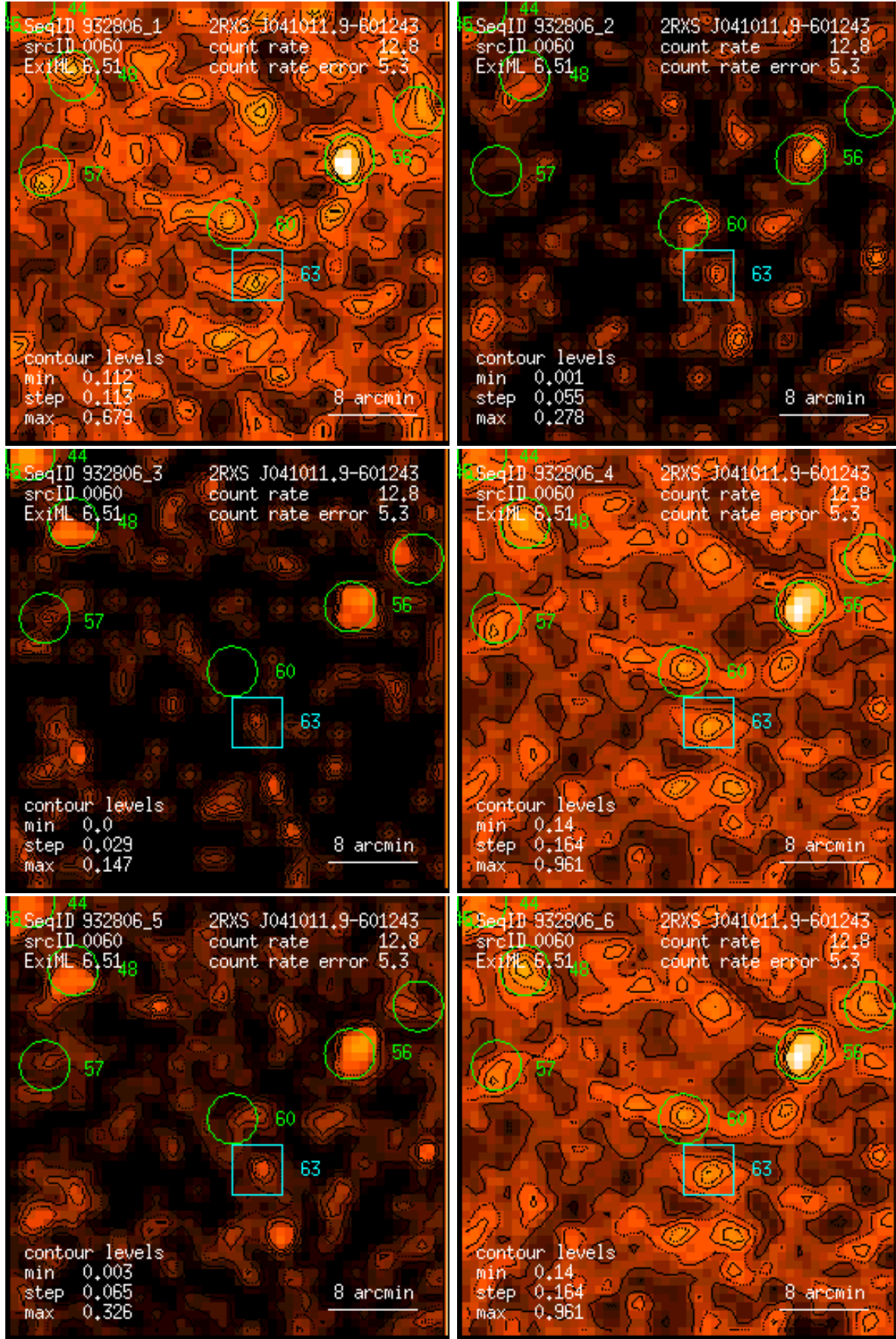
Figure 60: RASS 932806: detection 0060: band rate images, Gaussian filter: (1) PSPC channels 11 – 41, (2) 52 – 90, (3) 91 – 201, (4) 11 – 235, (5) 52 – 201, (6) 11 – 201. Broad band rates in counts/ks. Band rate contour levels in counts/ks/arcmin 2 .
