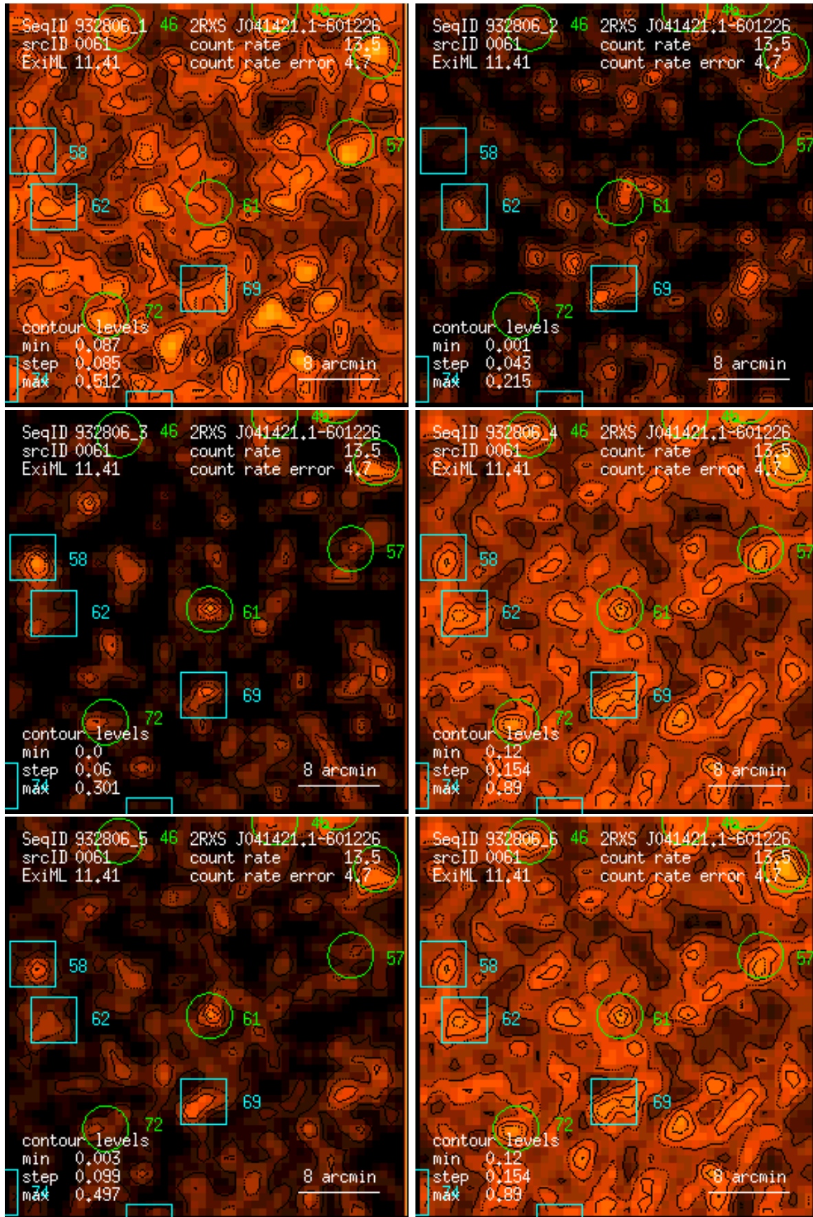
Figure 61: RASS 932806: detection 0061: band rate images, Gaussian filter: (1) PSPC channels 11 – 41, (2) 52 – 90, (3) 91 – 201, (4) 11 – 235, (5) 52 – 201, (6) 11 – 201. Broad band rates in counts/ks. Band rate contour levels in counts/ks/arcmin 2 .
