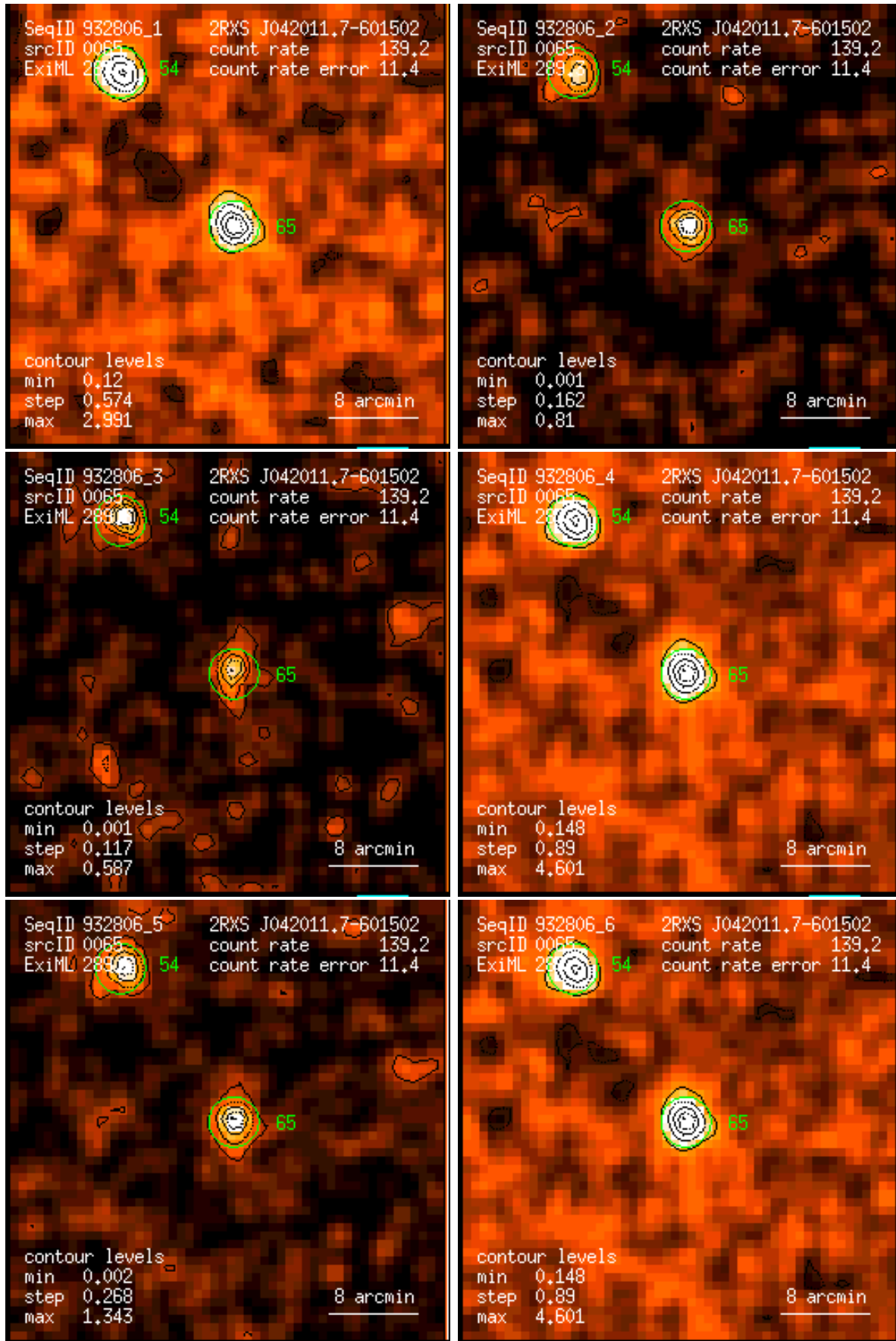
Figure 65: RASS 932806: detection 0065: band rate images, Gaussian filter: (1) PSPC channels 11 – 41, (2) 52 – 90, (3) 91 – 201, (4) 11 – 235, (5) 52 – 201, (6) 11 – 201. Broad band rates in counts/ks. Band rate contour levels in counts/ks/arcmin 2 .
