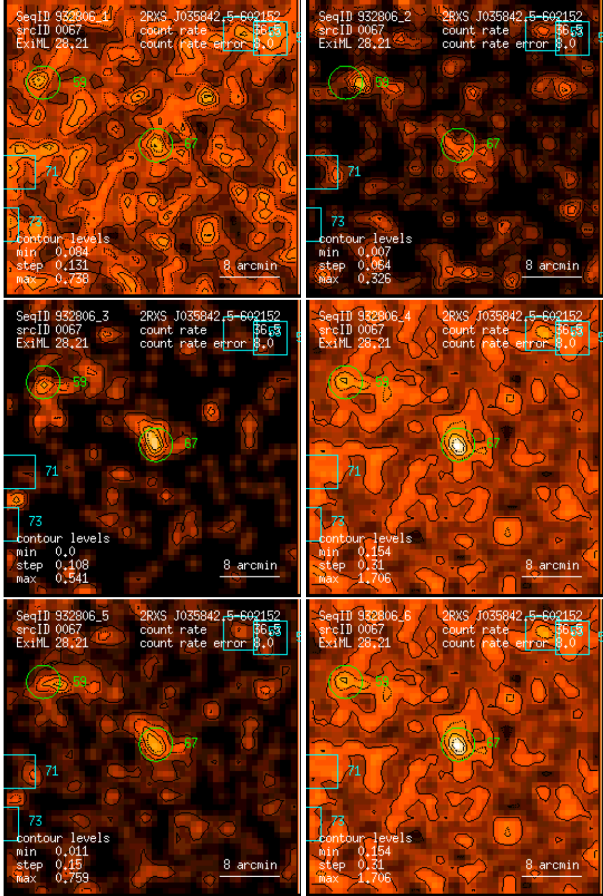
Figure 67: RASS 932806: detection 0067: band rate images, Gaussian filter: (1) PSPC channels 11 – 41, (2) 52 – 90, (3) 91 – 201, (4) 11 – 235, (5) 52 – 201, (6) 11 – 201. Broad band rates in counts/ks. Band rate contour levels in counts/ks/arcmin 2 .
