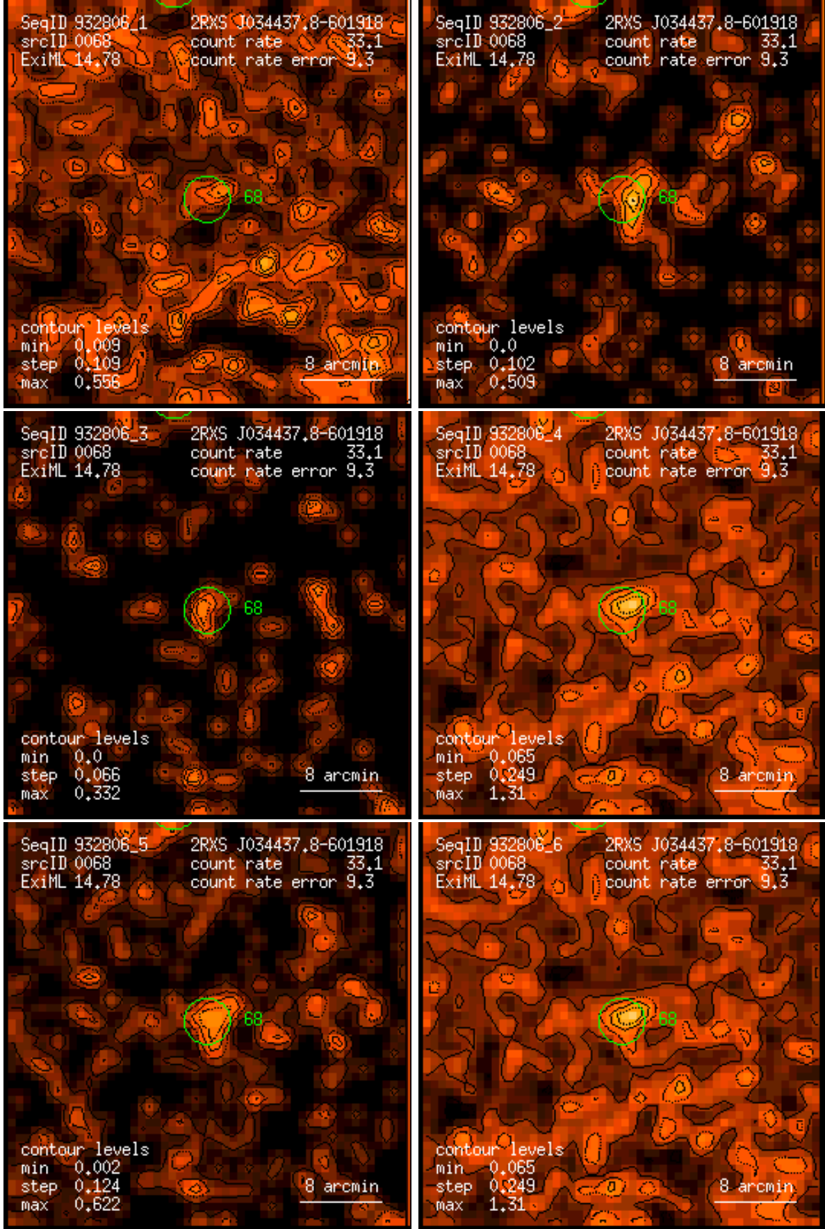
Figure 68: RASS 932806: detection 0068: band rate images, Gaussian filter: (1) PSPC channels 11 – 41, (2) 52 – 90, (3) 91 – 201, (4) 11 – 235, (5) 52 – 201, (6) 11 – 201. Broad band rates in counts/ks. Band rate contour levels in counts/ks/arcmin 2 .
