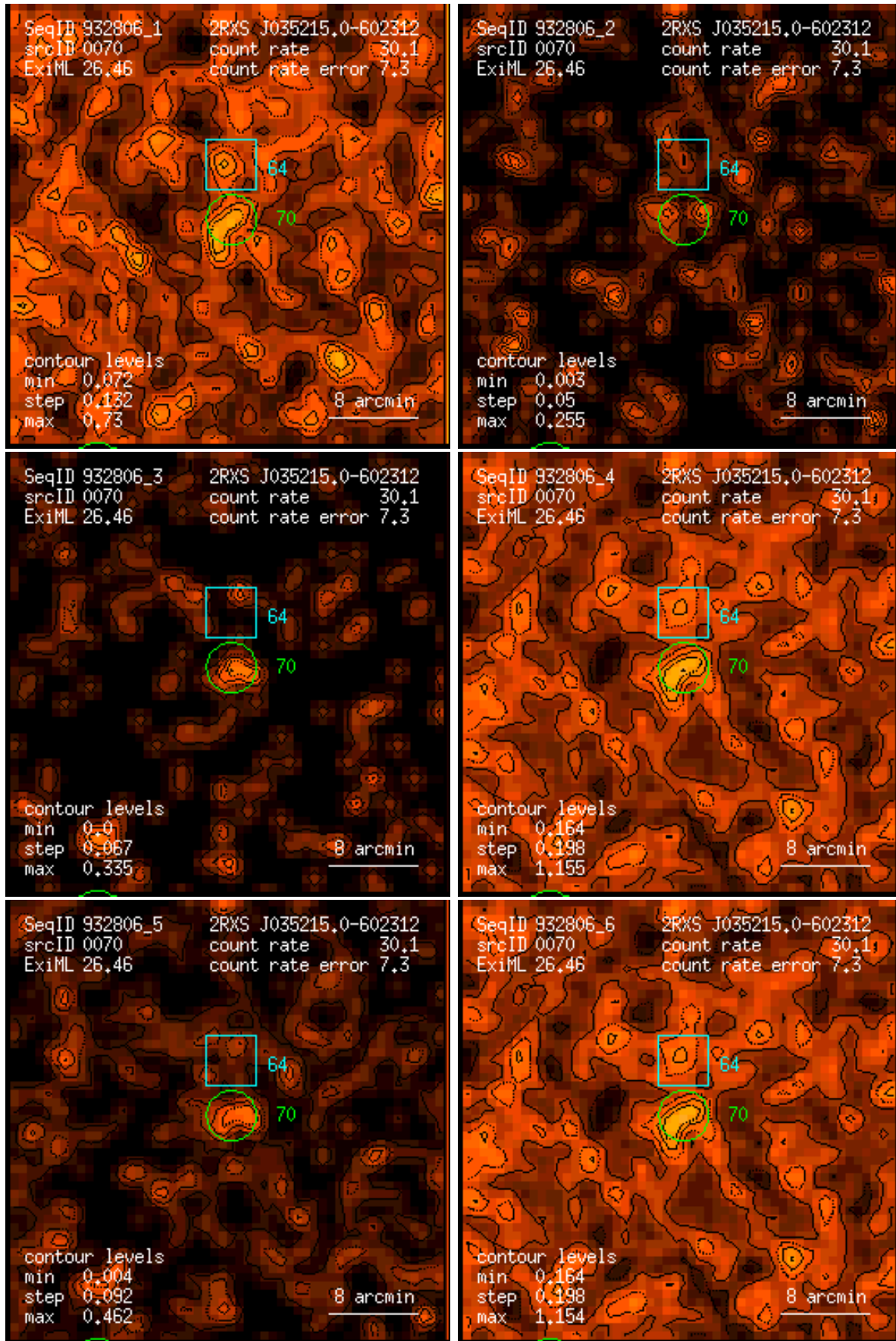
Figure 70: RASS 932806: detection 0070: band rate images, Gaussian filter: (1) PSPC channels 11 – 41, (2) 52 – 90, (3) 91 – 201, (4) 11 – 235, (5) 52 – 201, (6) 11 – 201. Broad band rates in counts/ks. Band rate contour levels in counts/ks/arcmin 2 .
